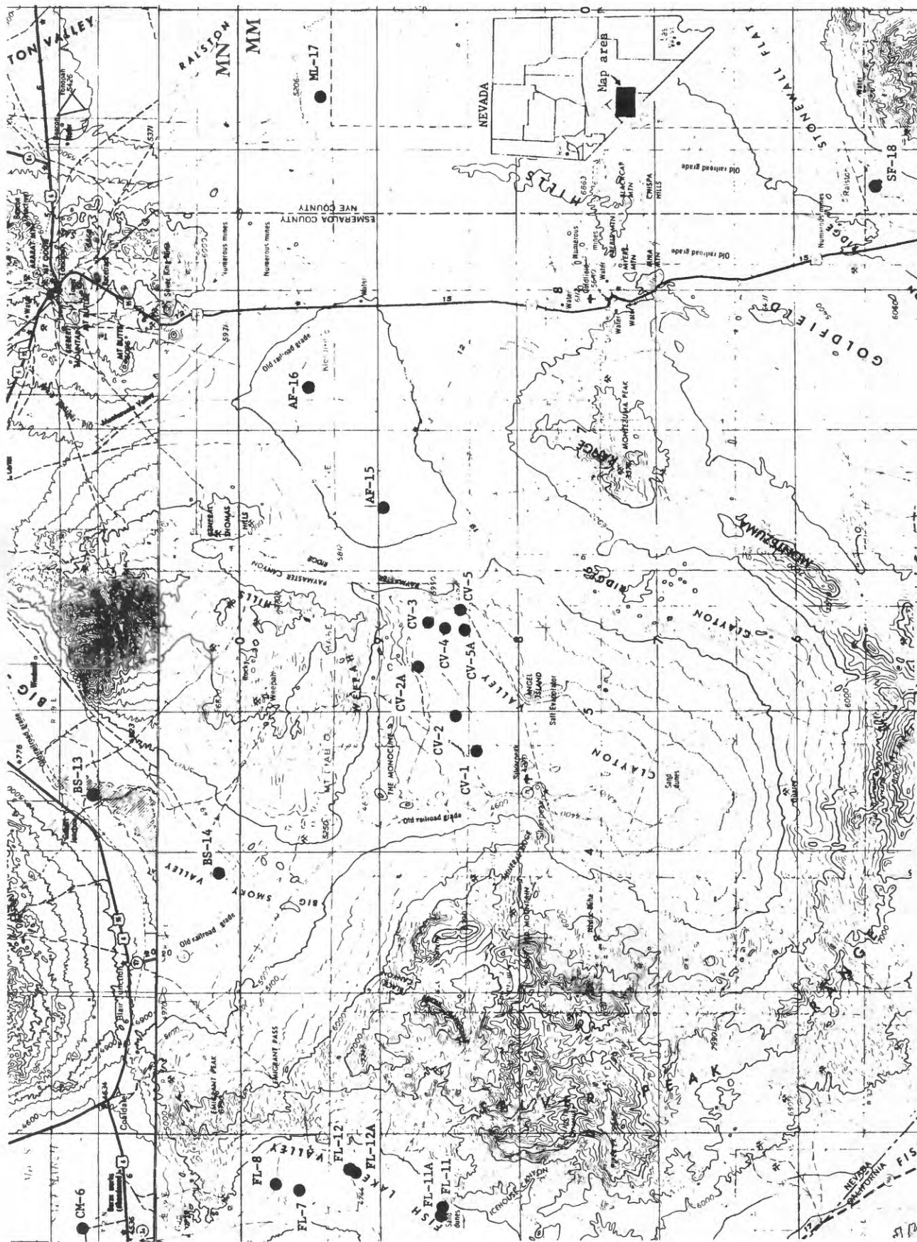
FIGURE 1.--Index map of a part of Esmeralda and Nye Counties, Nevada, showing location of drill sites. Base from the Goldfield and Tonopah 250,000 scale maps.
