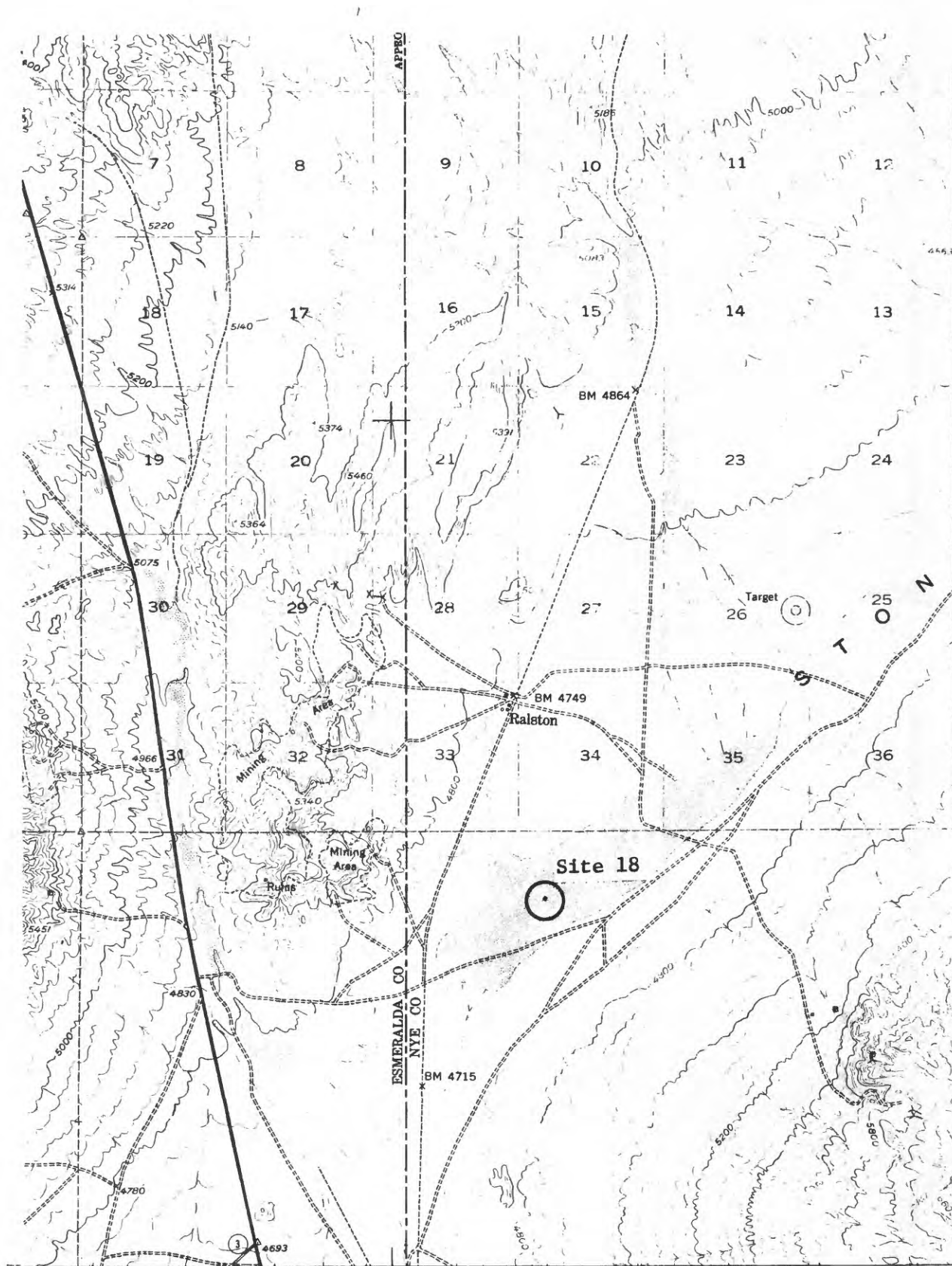
FIGURE 7.-- Map of a part of the Goldfield Quadrangle, Nye County, Nevada, Showing location of drill site 18. Scale: 1:62,500.
