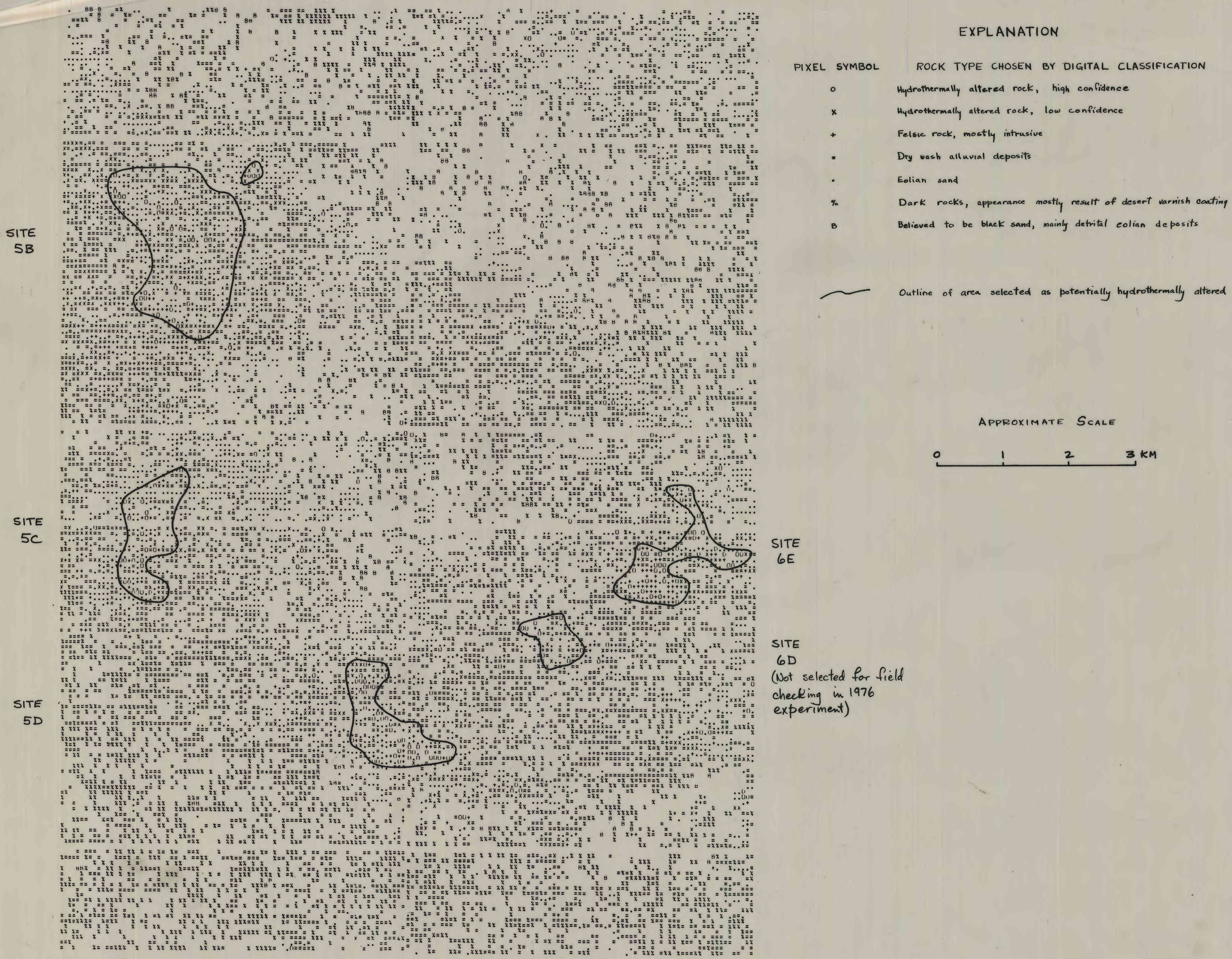
Figure 5: Digital classification map of stratovolcano area
