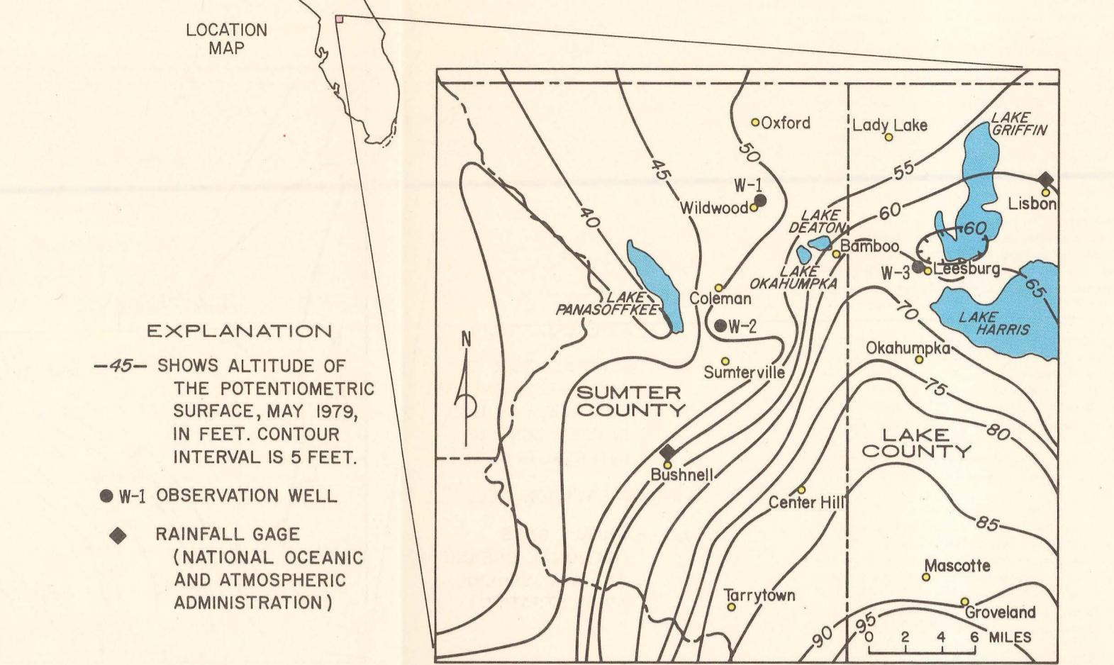
Figure 1.—Sumter-west Lake County area showing locations of selected hydrologic record stations, and the potentiometric surface of the Floridan aquifer for May 1979. (Laughlin, Hayes, and Schiner, 1979)
