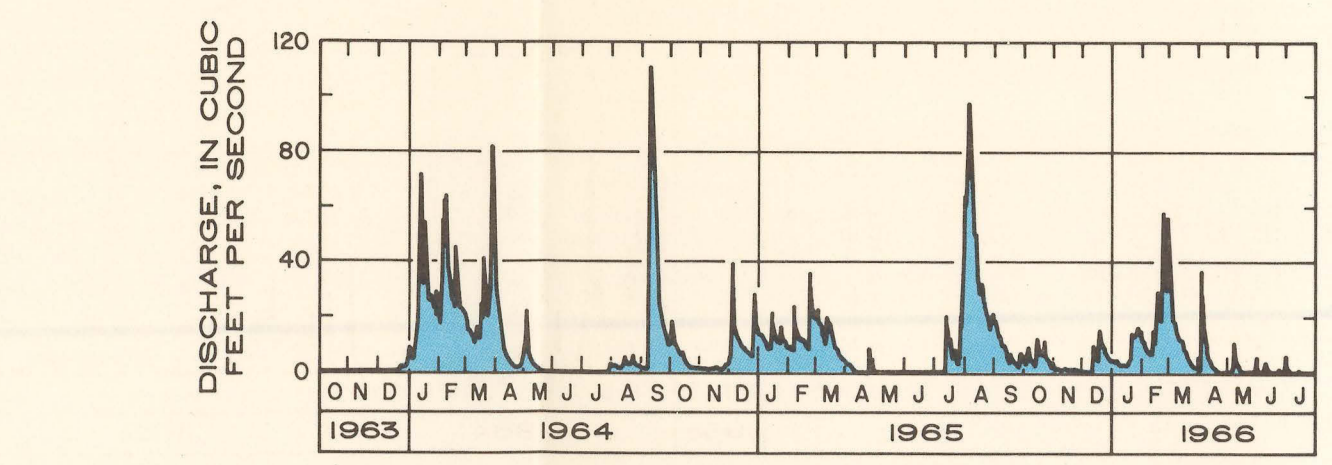
Figure 7.—Discharge of Chitty Chatty Creek for the period October 1963 to July 1966.
