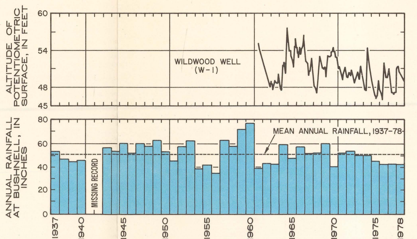
Figure 5.—Long-term rainfall at Bushnell and elevation of potentiometric surface of the Floridan aquifer near Wildwood.
