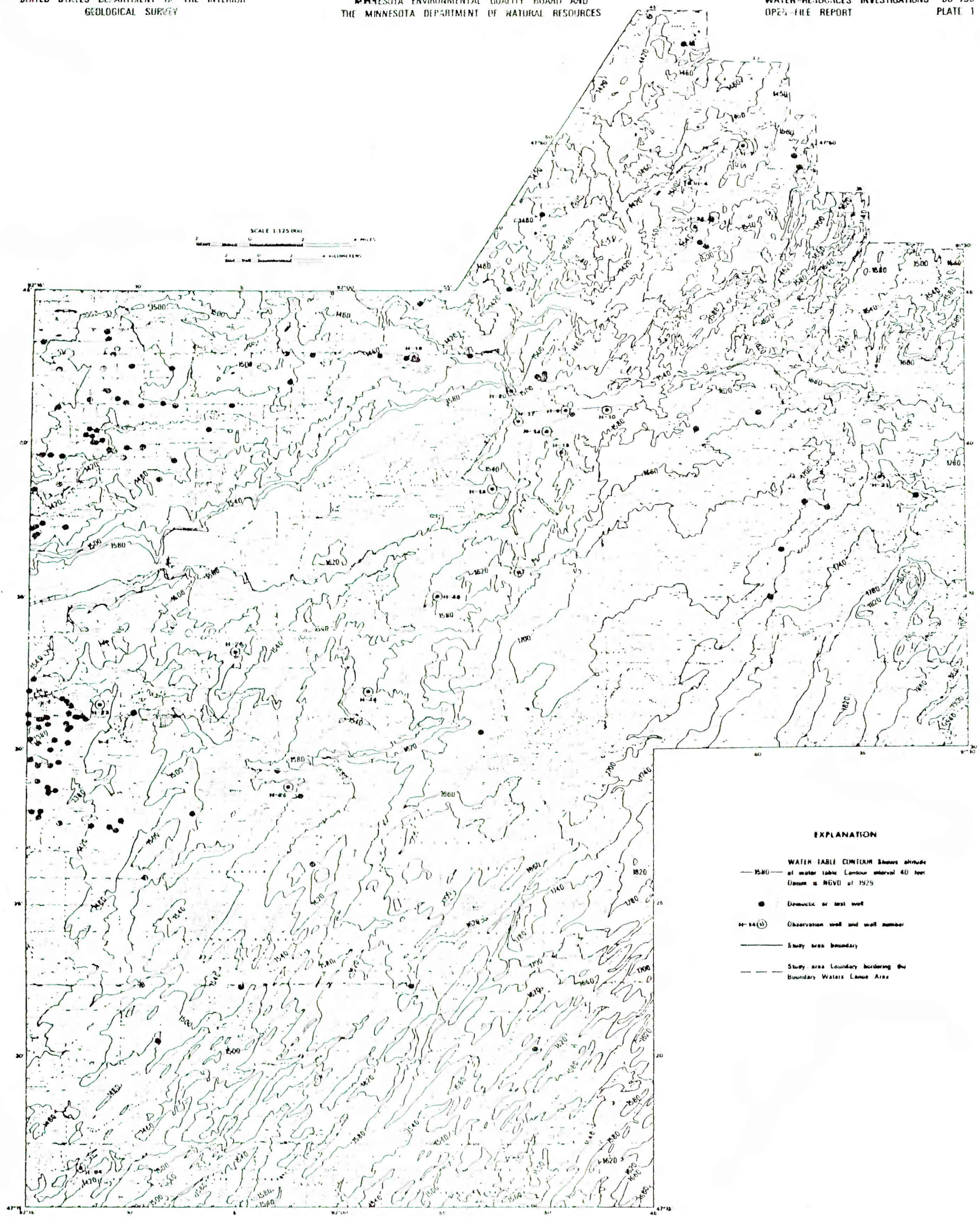
PLATE 1.—GENERALIZED MAP OF THE WATER TABLE IN THE COPPER-NICKEL STUDY REGION, NORTHEASTERN MINNESOTA
