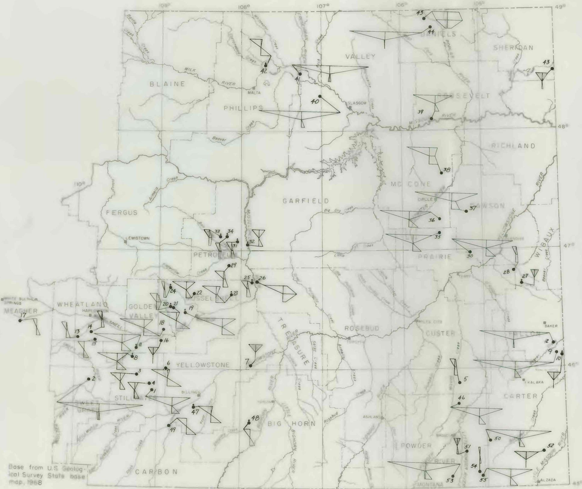
Figure 4.—Stiff diagrams of selected analyses of water from rocks of Cretaceous age.
