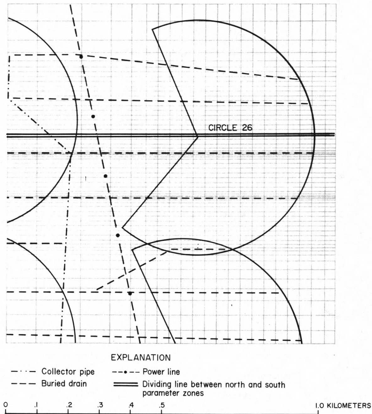
Figure 3.--Finite-difference grid spacings and parameter zones used in parameter estimation model.
