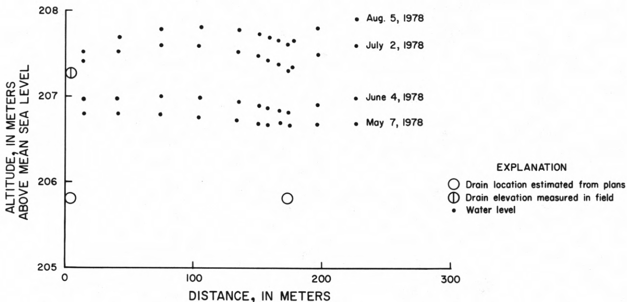
Figure 8.--Relation of water levels to two drains in irrigation circle 33 in spring and summer 1978.
