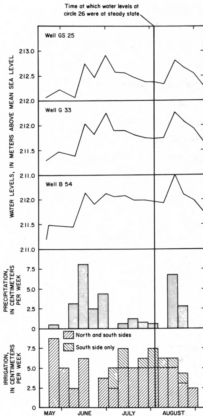
Figure 4.--Precipitation, irrigation, and water levels during the summer of 1978.
