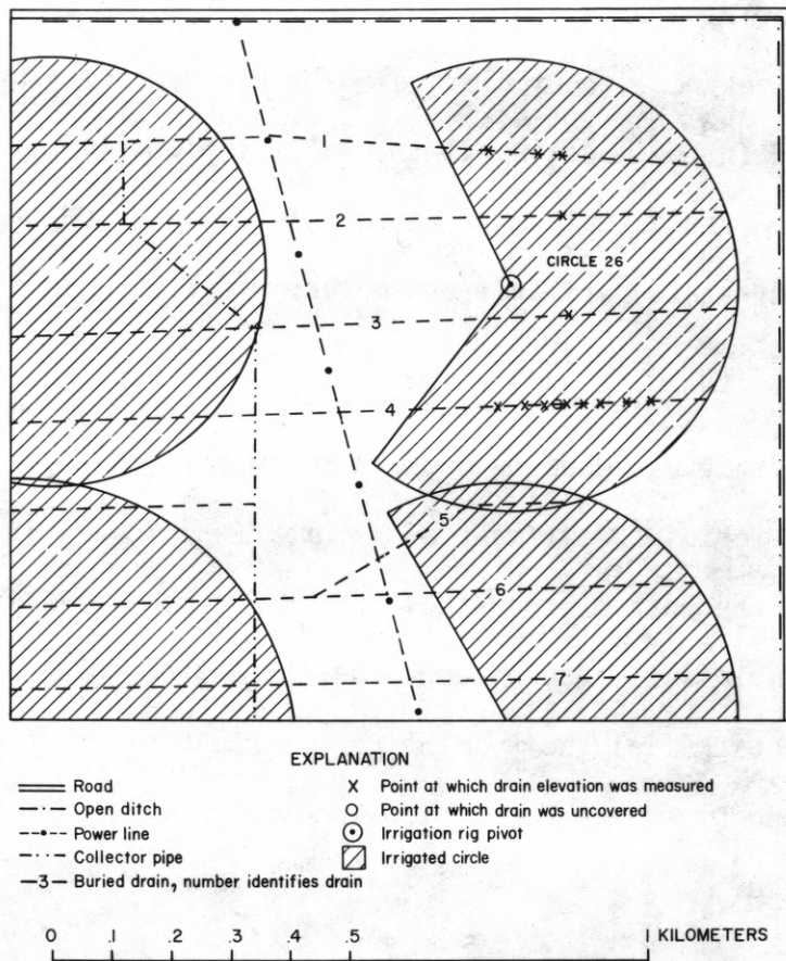
Figure 2.--Irrigation circle 26 and adjoining circles.
