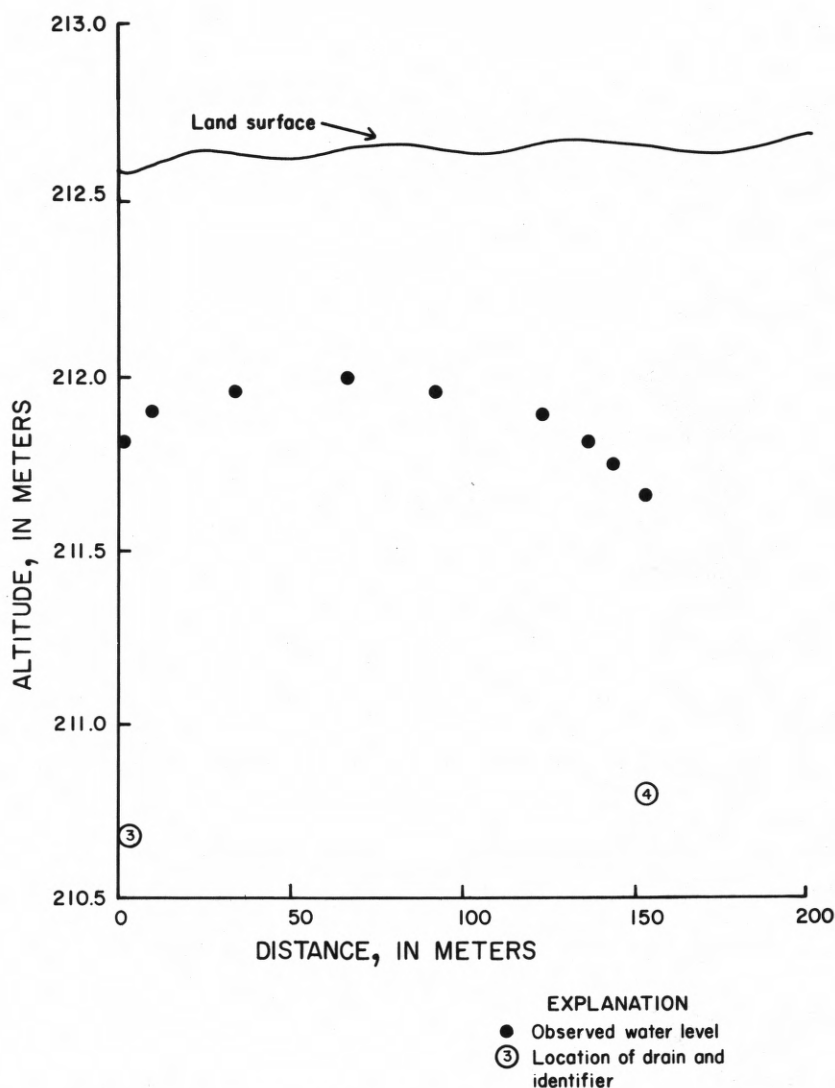
Figure 9.--Relation of water levels to drains in a cross section perpendicular to two drains in irrigation circle 26 in August 1978.
