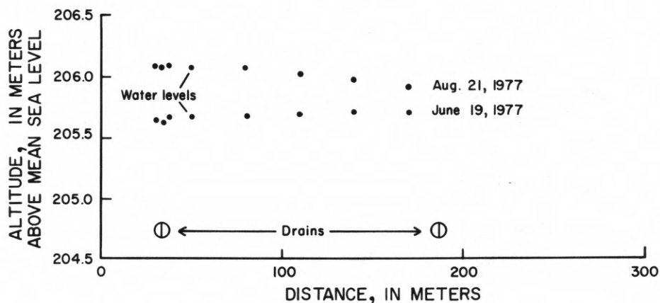
Figure 7.--Relation of water levels to two drains in irrigation circle 47 in June and August 1977.
