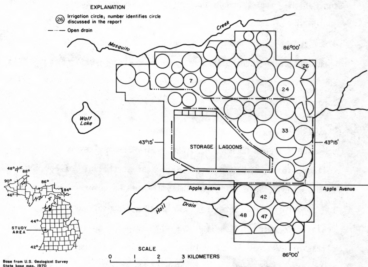
Figure 1.--Muskegon County wastewater management system.
