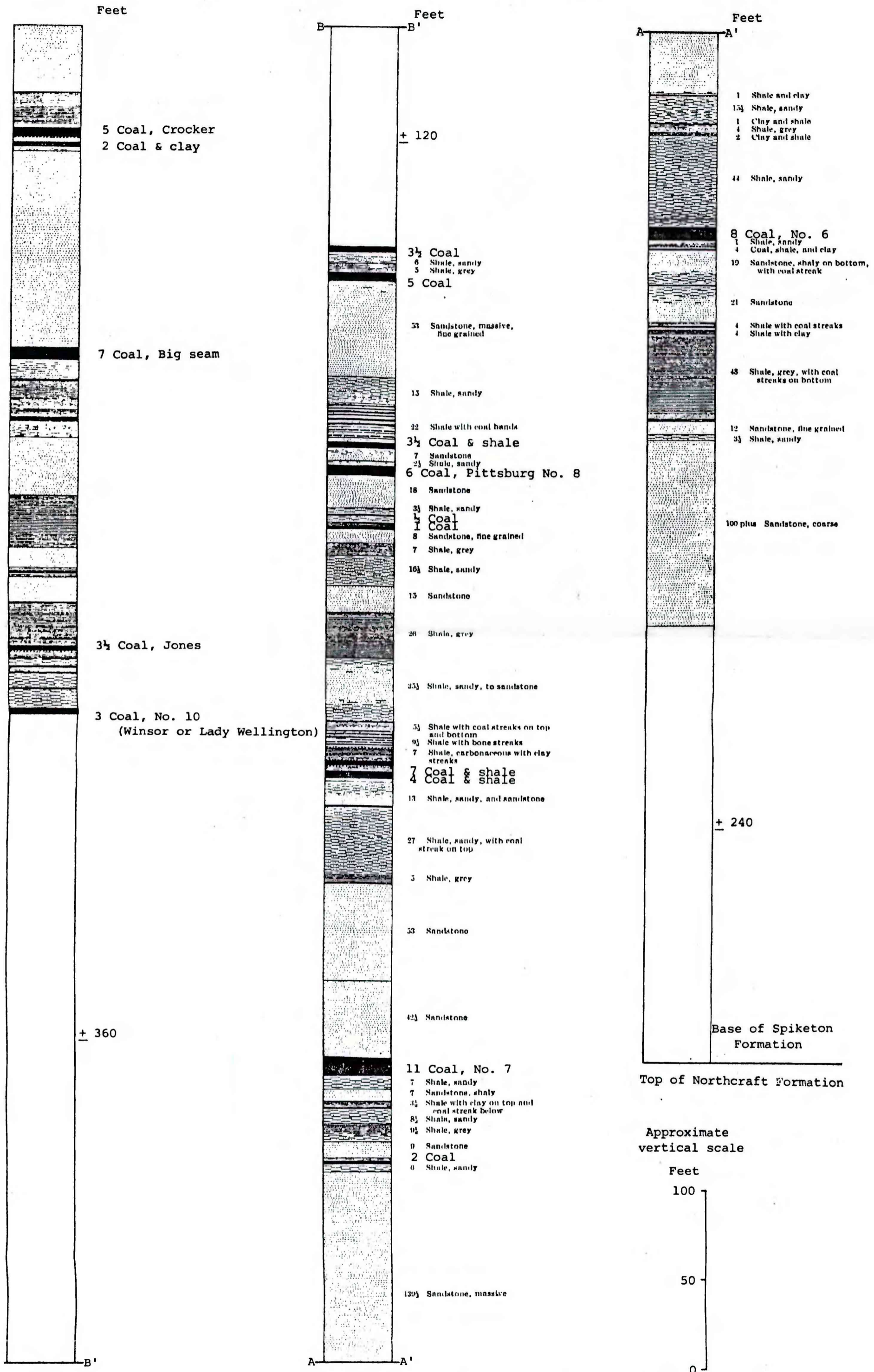
FIGURE 24.--Generalized columnar section of the Spiketon Formation at Spiketon and South Willis mines. (modified from Daniels, 1914, pl. 16)
