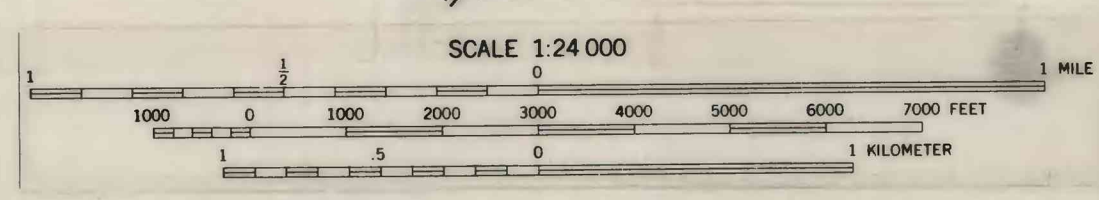
PRELIMINARY GEOLOGIC MAP OF THE CLEAR LAKE SW QUADRANGLE, WASHINGTON By D.P. Dethier and J.T. Whetten 1980
