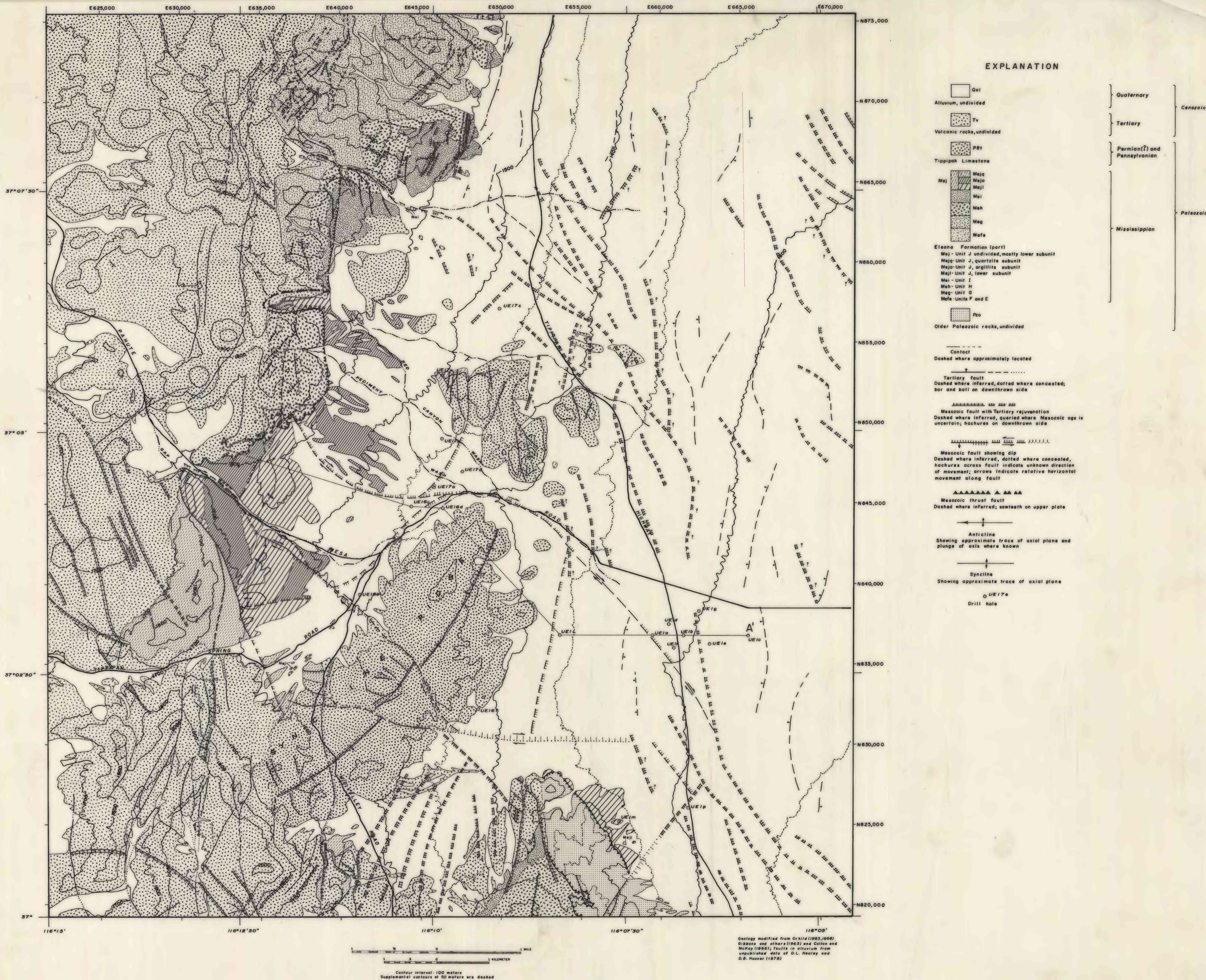
Figure 3.--Geologic map of the Syncline Ridge area
