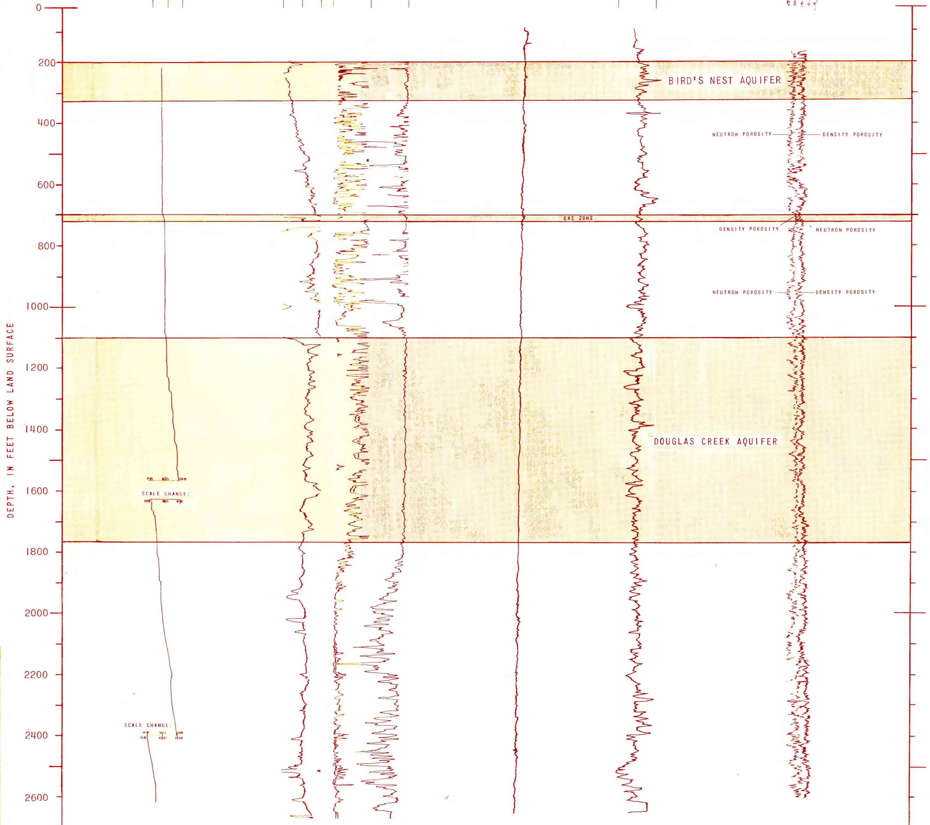
PLATE I.--WATER-TEMPERATURE AND GEOPHYSICAL LOGS OF TEST HOLE I SHOWING MAJOR WATER-BEARING ZONES, SOUTHEASTERN UINTA BASIN, UTAH.
