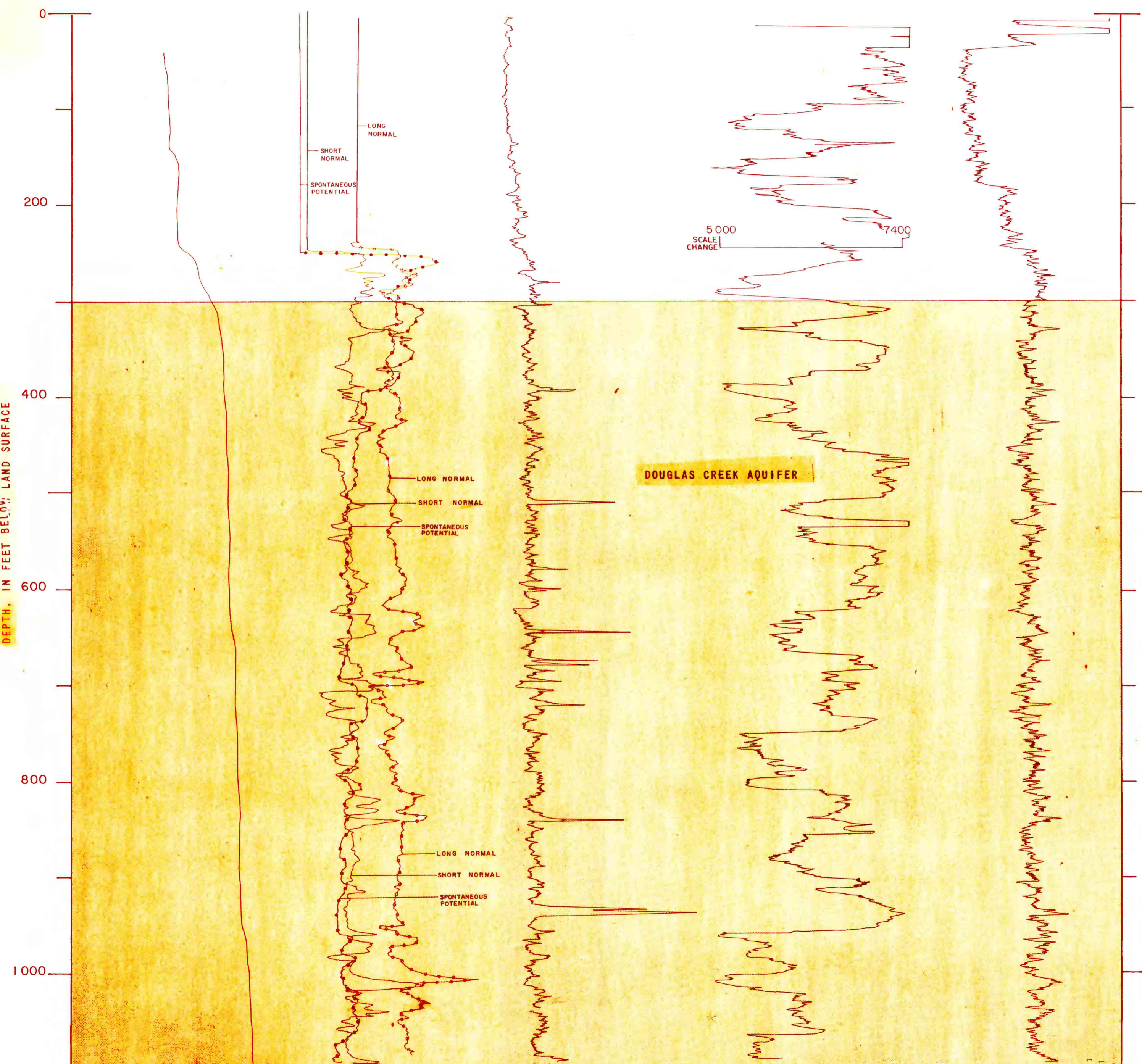
PLATE 3.--WATER-TEMPERATURE AND GEOPHYSICAL LOGS OF TEST HOLE 3 SHOWING MAJOR WATER-BEARING ZONES, SOUTHEASTERN UINTA BASIN, UTAH.
