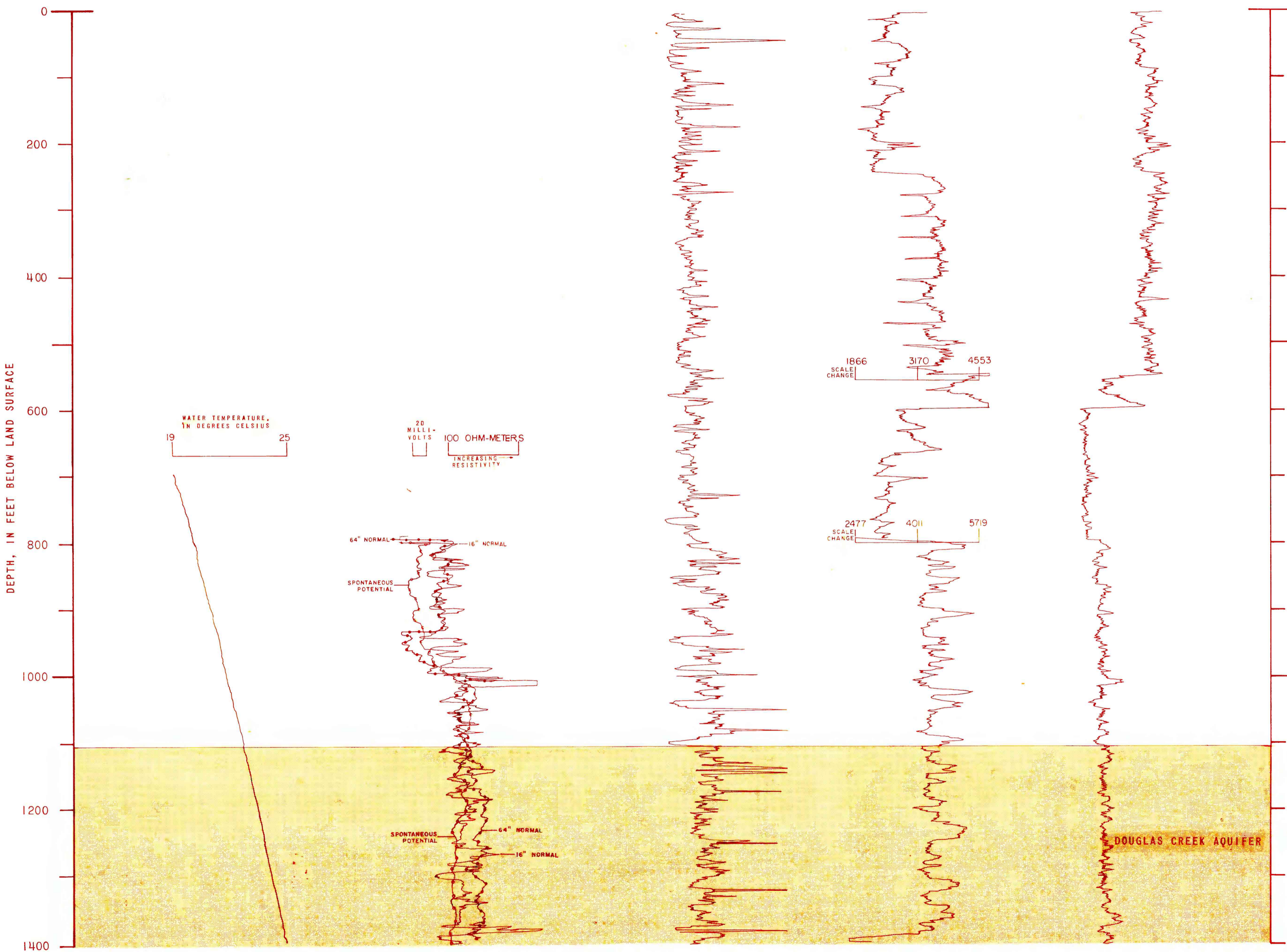
PLATE 4.--WATER-TEMPERATURE AND GEOPHYSICAL LOGS OF TEST HOLE 4 SHOWING MAJOR WATER-BEARING ZONES, SOUTHEASTERN UINTA BASIN, UTAH.
