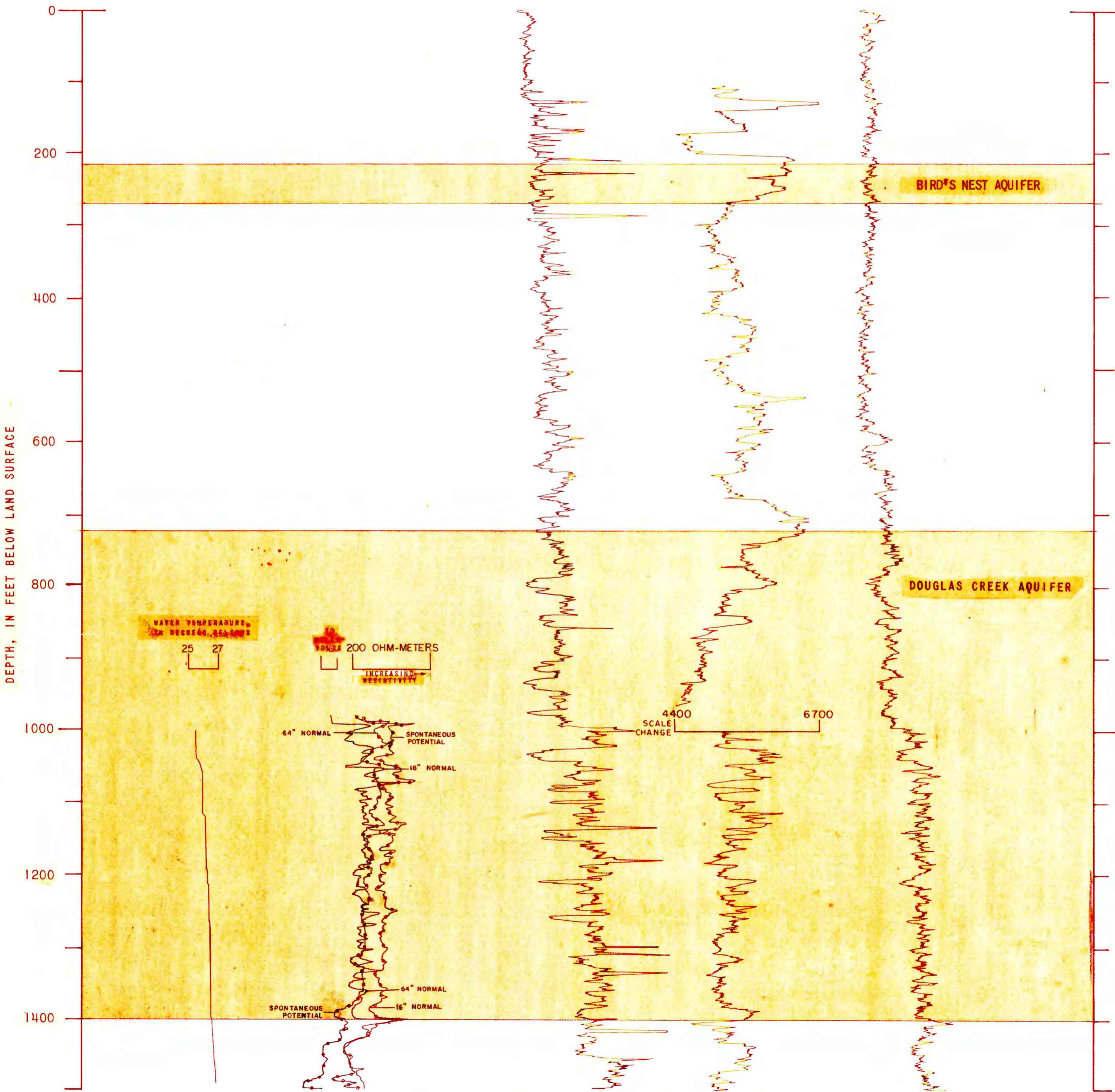
PLATE 6.--WATER-TEMPERATURE AND GEOPHYSICAL LOGS OF TEST HOLE 6 SHOWING MAJOR WATER-BEARING ZONES, SOUTHEASTERN UINTA BASIN, UTAH.
