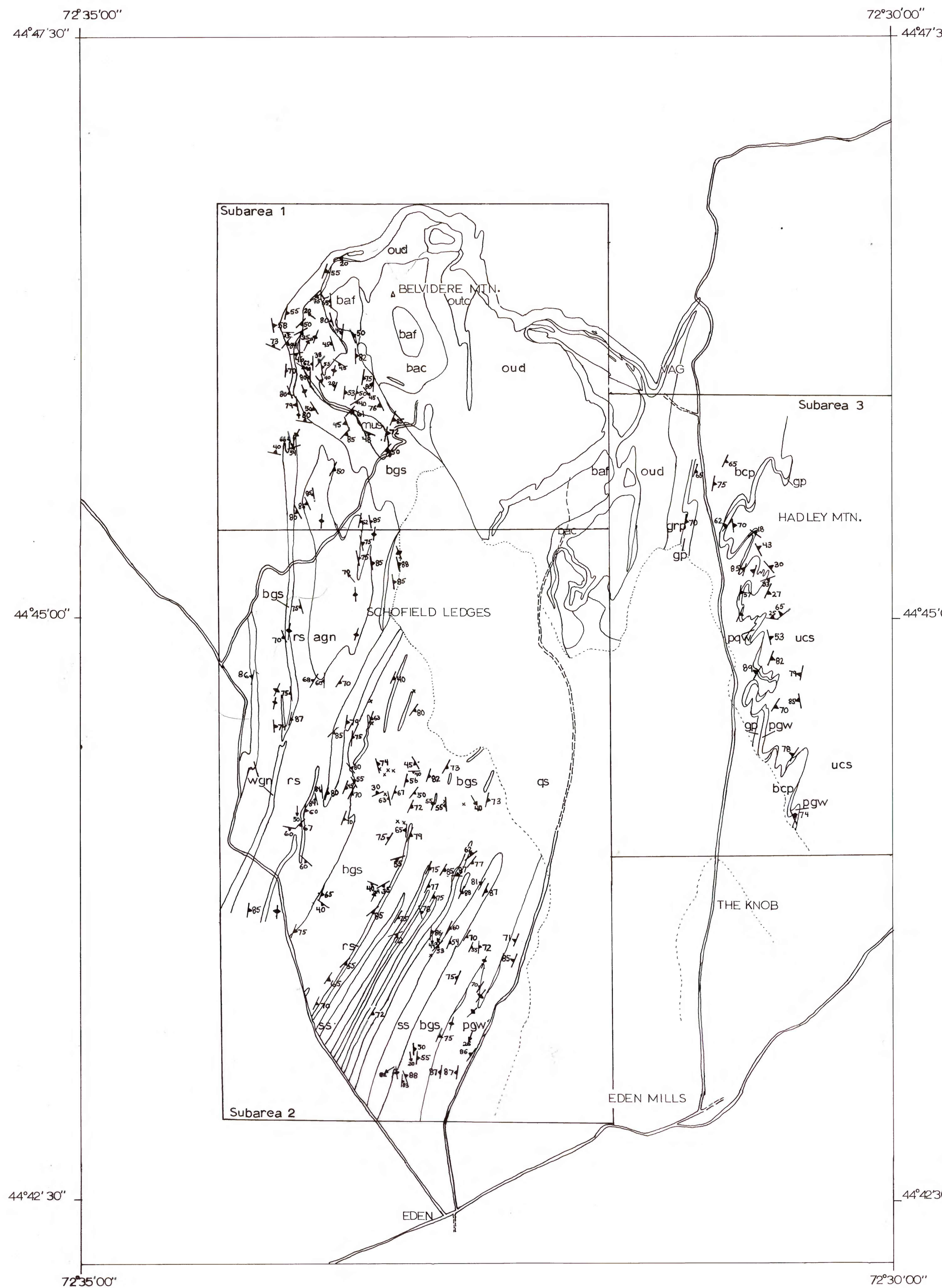
PLATE IV F2 STRUCTURE MAP
