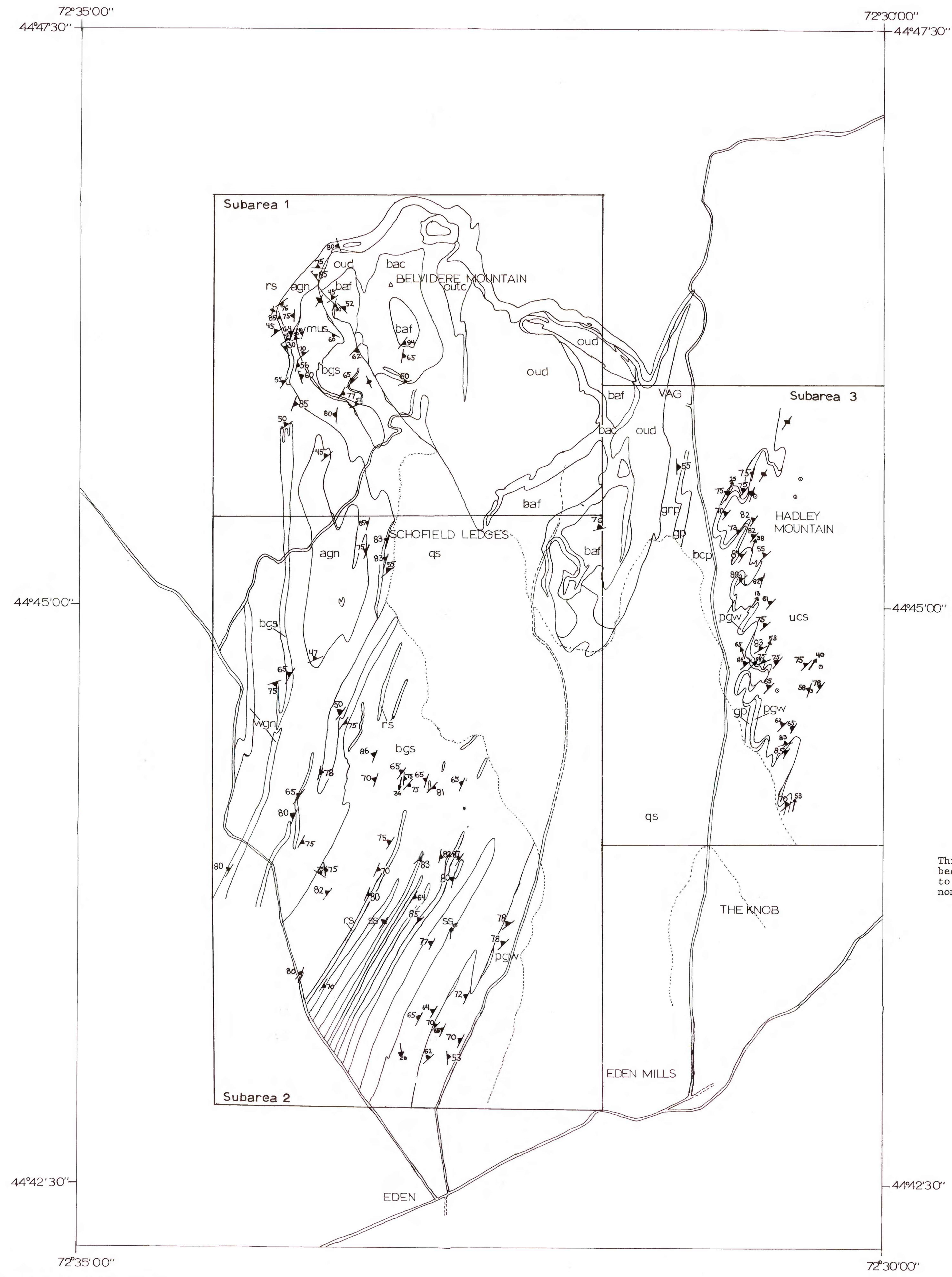
PLATE V F3 STRUCTURE MAP
