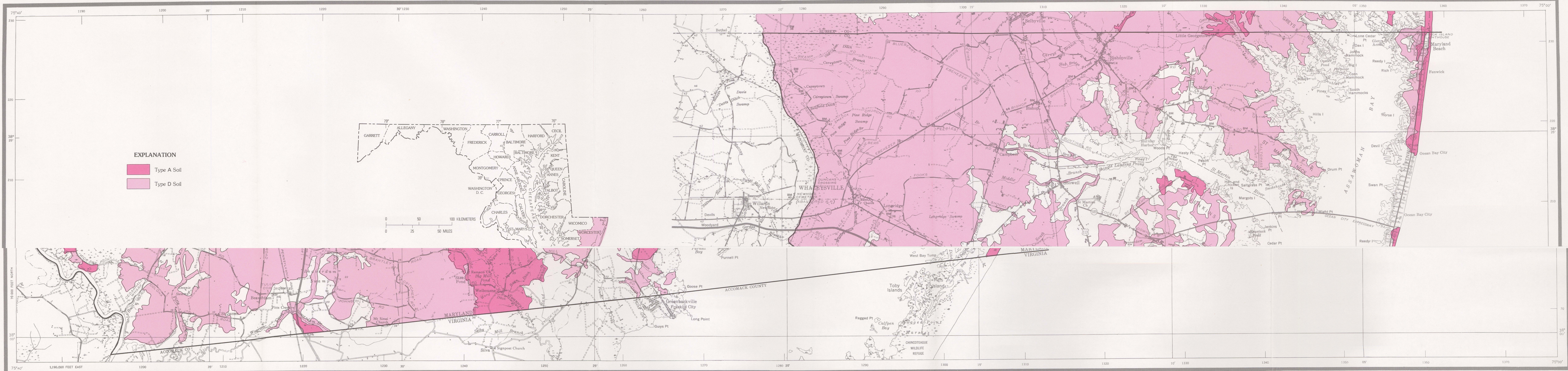
MAP SHOWING EXTENT OF TYPE A AND TYPE D SOILS, WORCESTER COUNTY, MARYLAND
