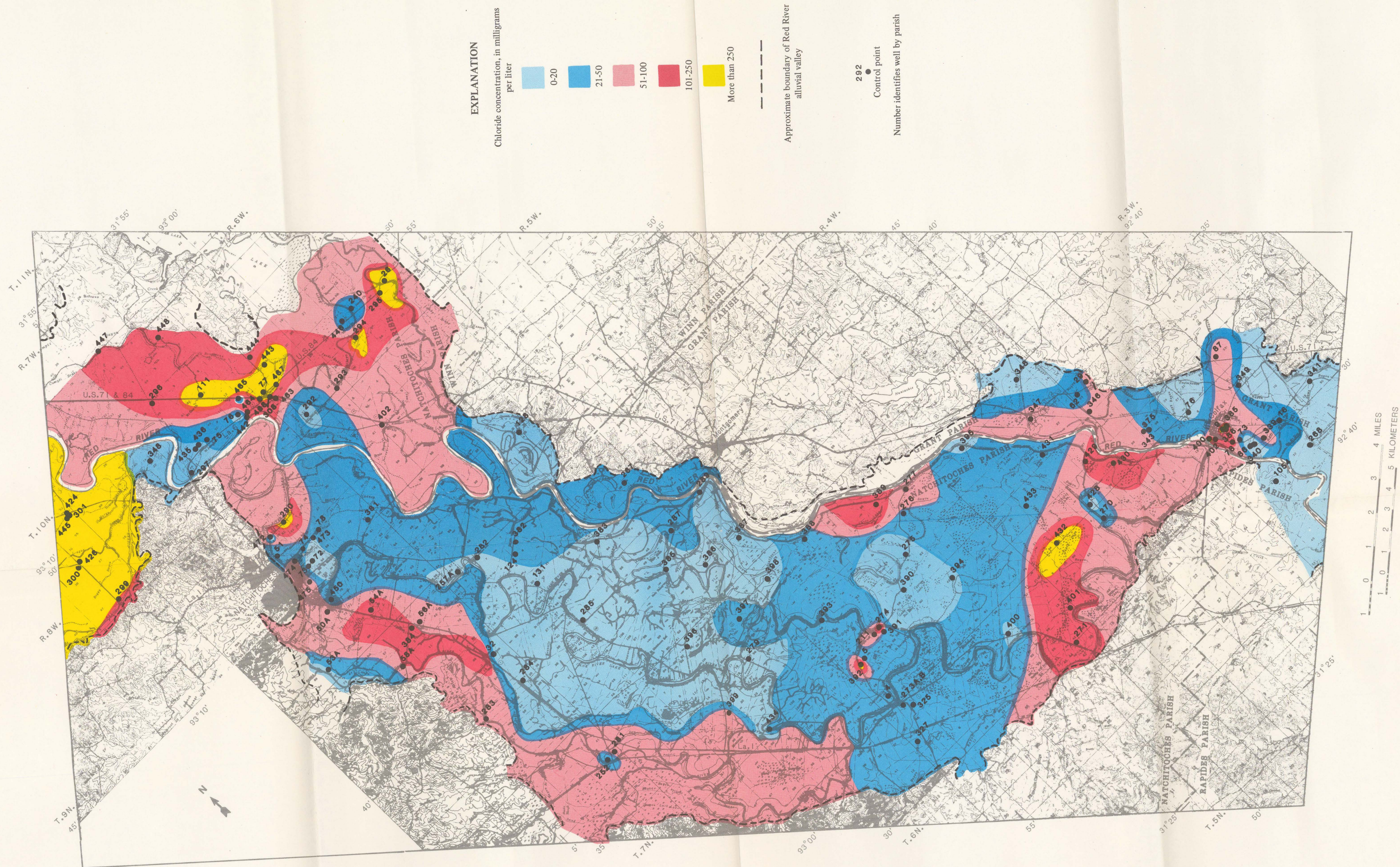
PLATE 14. MAP SHOWING DISTRIBUTION OF CHLORIDE IN WATER FROM THE RED RIVER ALLUVIAL AQUIFER, NATCHITOCHES-COLFAX AREA, LOUISIANA.
