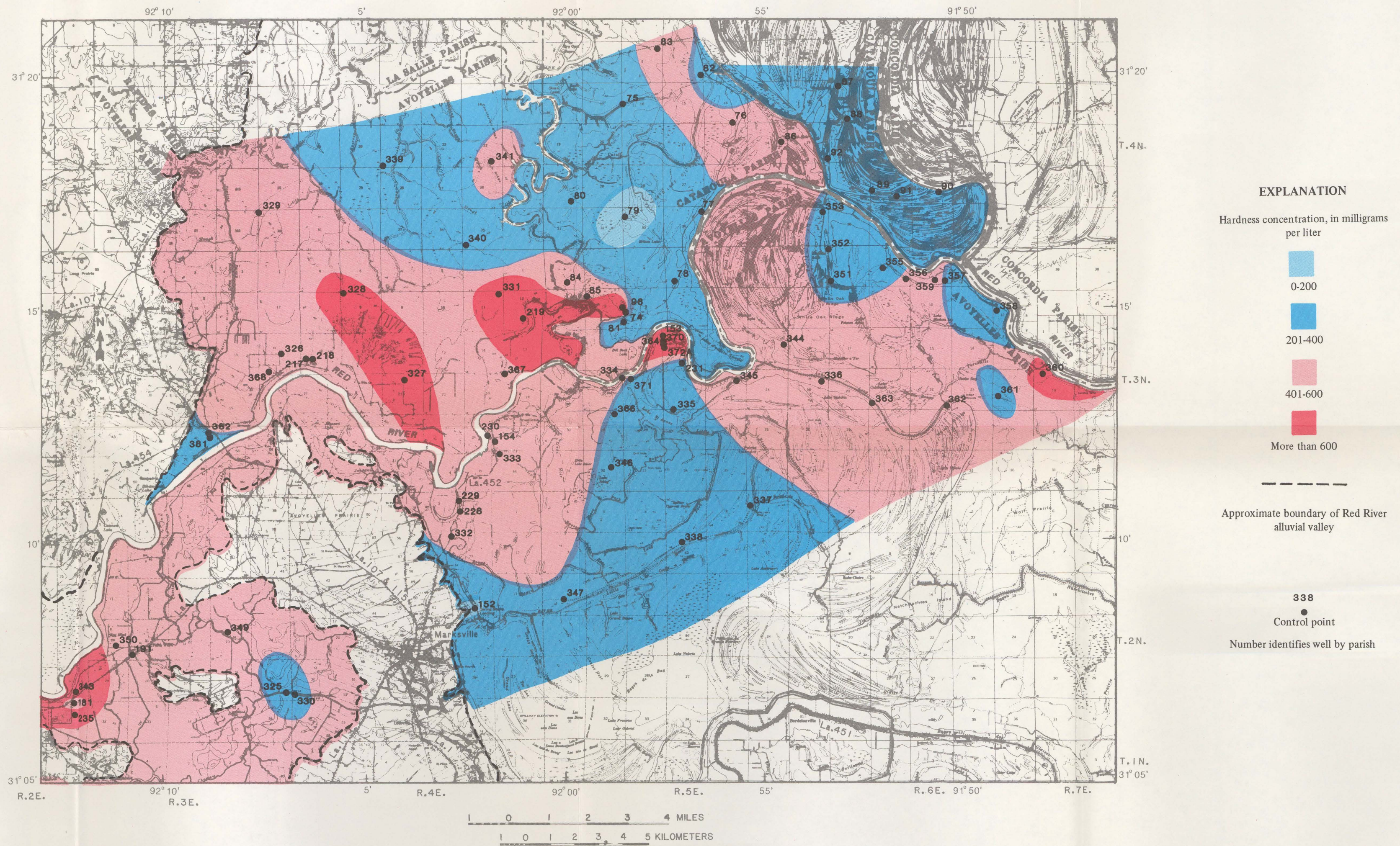
PLATE 6. MAP SHOWING DISTRIBUTION OF HARDNESS IN WATER FROM THE RED RIVER ALLUVIAL AQUIFER, MARKSVILLE AREA, LOUISIANA.
