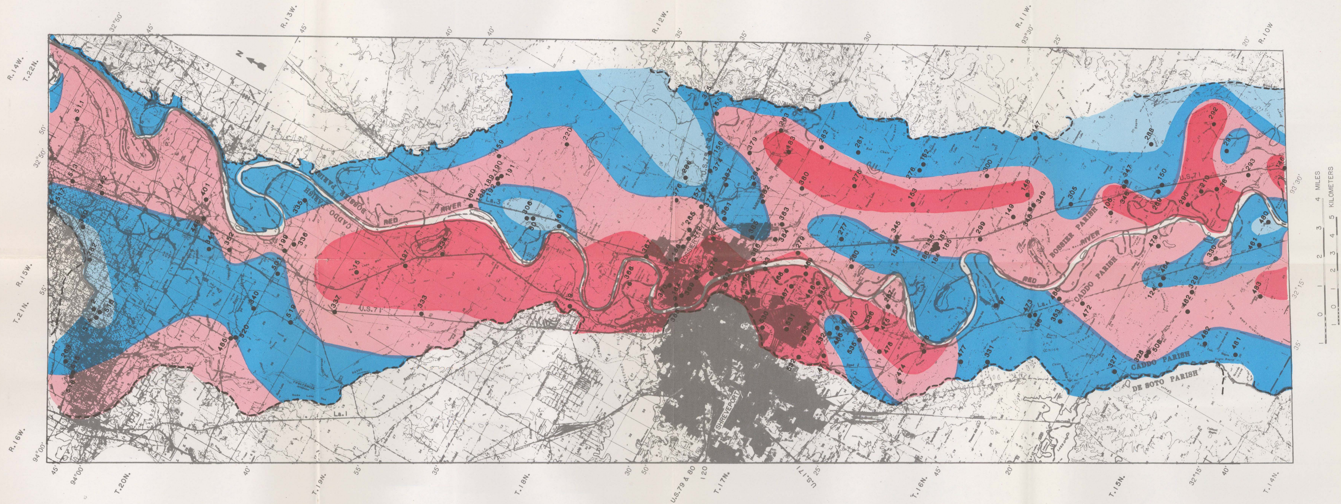
PLATE 7. MAP SHOWING DISTRIBUTION OF IRON IN WATER FROM THE RED RIVER ALLUVIAL AQUIFER, SHREVEPORT AREA, LOUISIANA.
