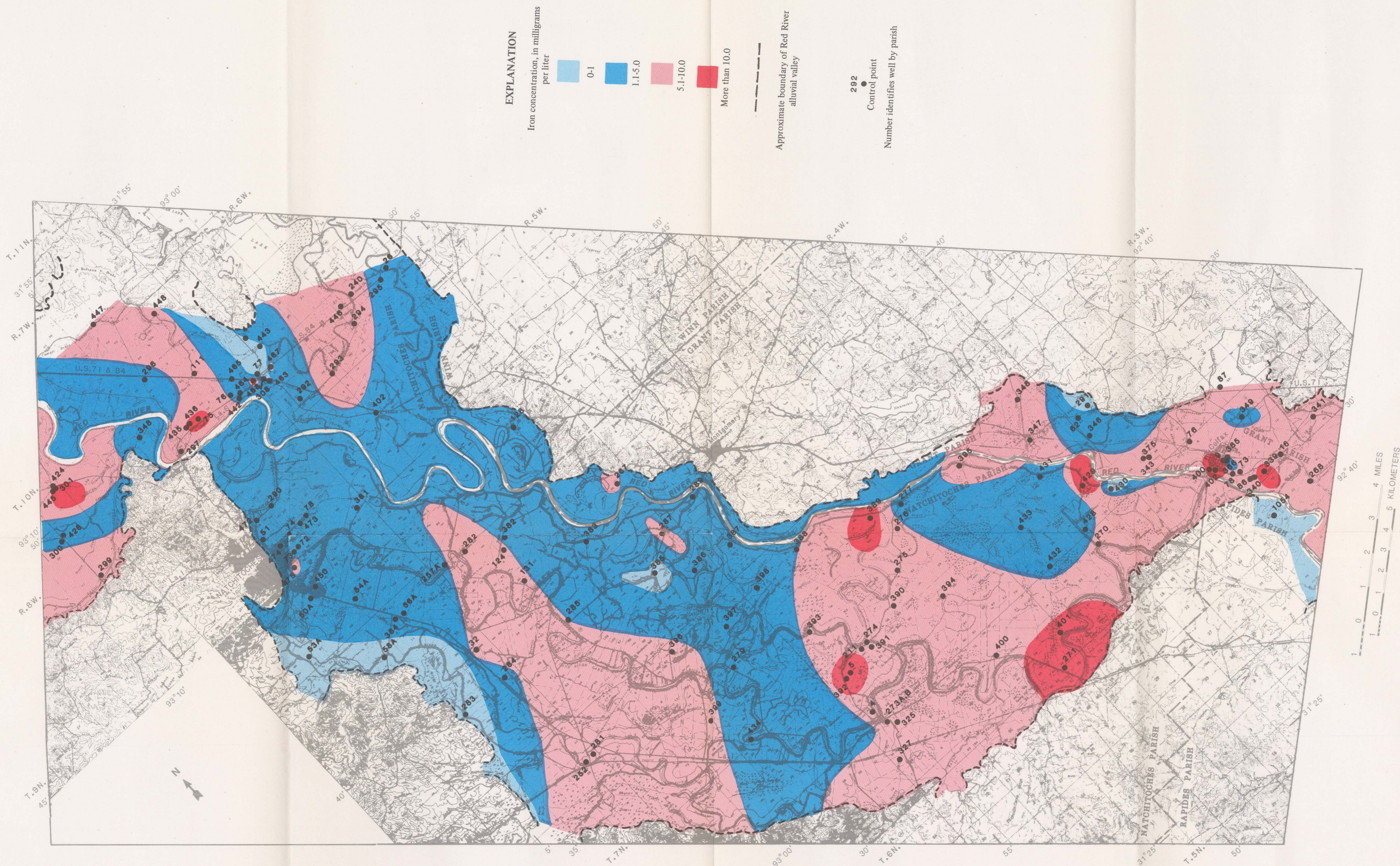
PLATE 9. MAP SHOWING DISTRIBUTION OF IRON IN WATER FROM THE RED RIVER ALLUVIAL AQUIFER, NATCHITOCHEs-COLFAx AREA, LOUISIANA.
