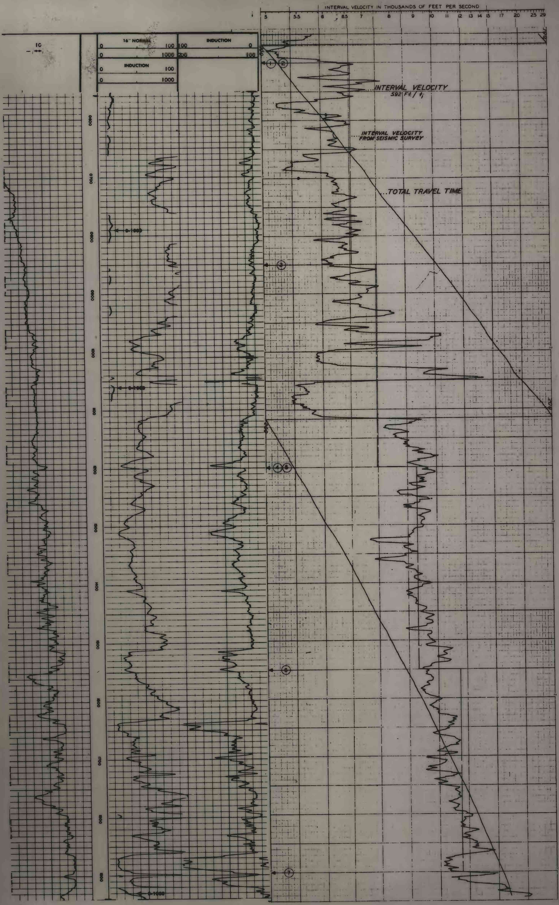
Figure 10.--Geophysical logs obtained in Hagestad drill hole.
