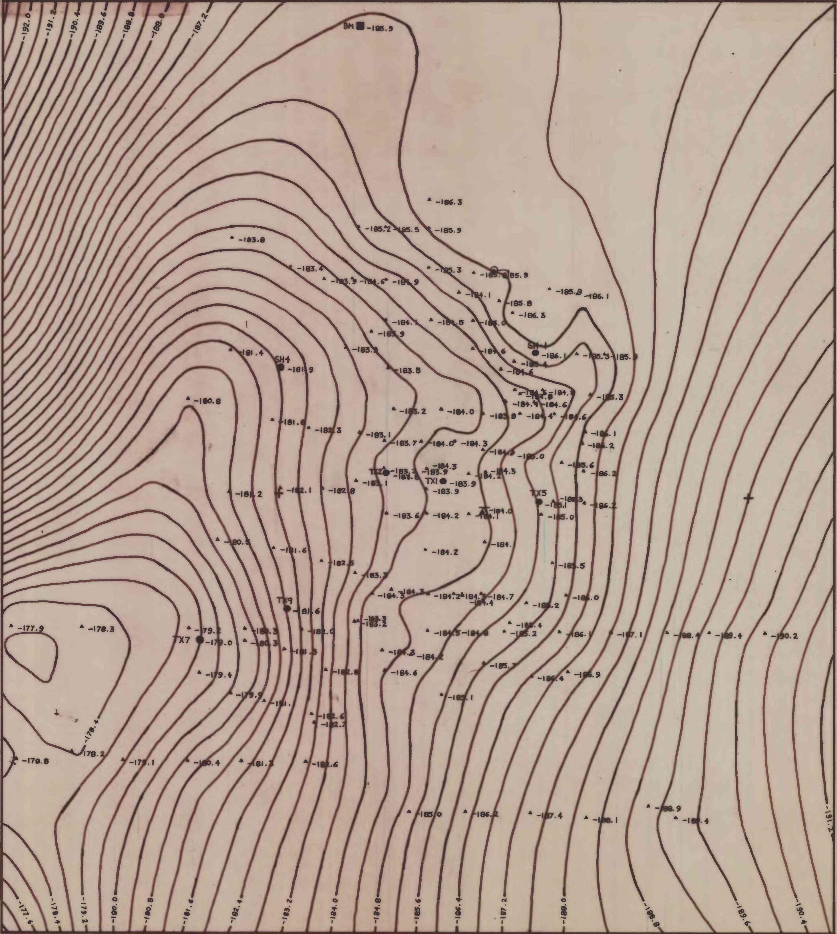
Appendix C - Bouguer gravity anomaly map of the Fm's Geothermal Area, Montana Scale 1:6,000
