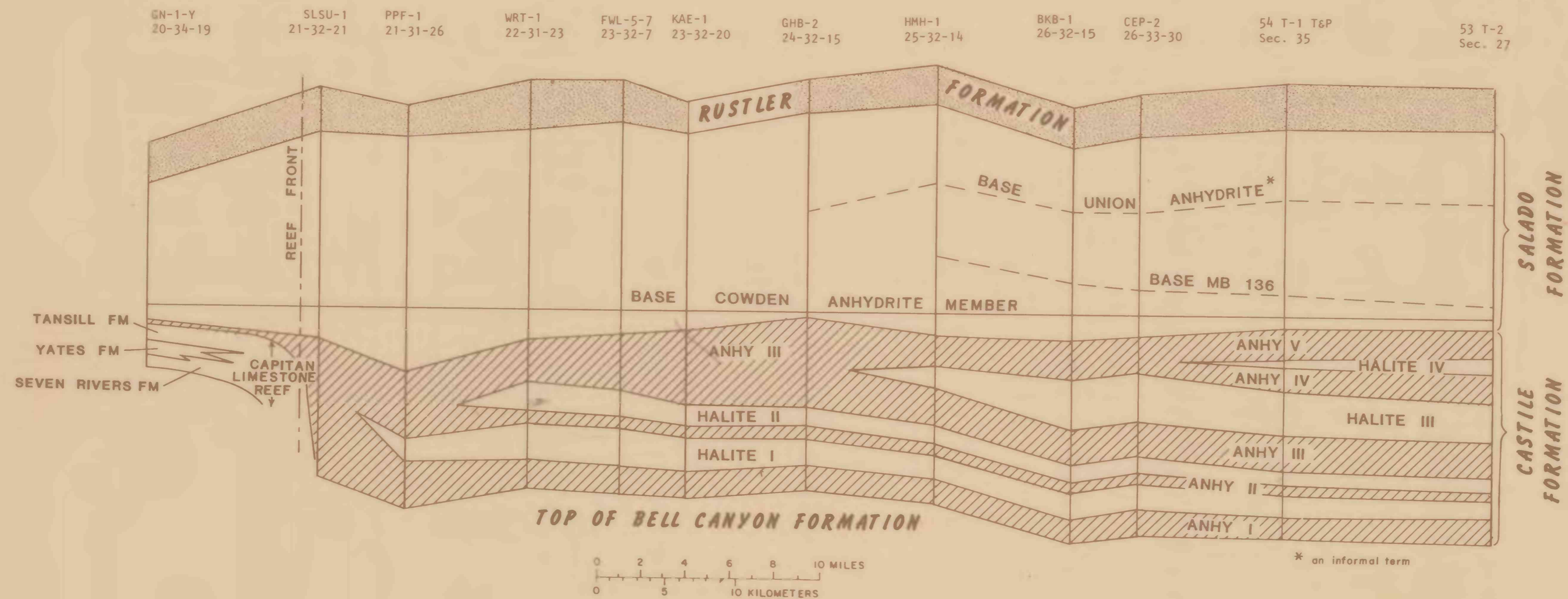
FIGURE 7.--CROSS SECTIONS OF CASTILE AND SALADO FORMATIONS, DELAWARE BASIN, SHOWING STRATIGRAPHIC RELATIONS (ANHY = ANHYDRITE).
