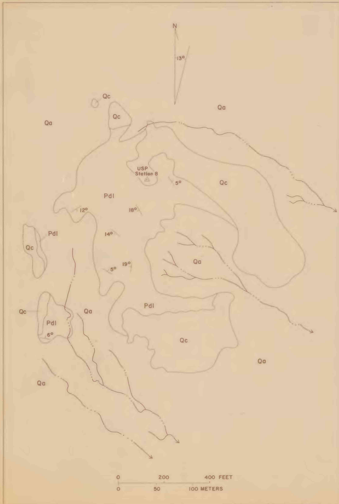
Figure 19.--Geologic sketch map of positive topographic feature, Nash Draw.
