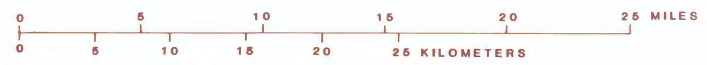
MAP SHOWING WATER-LEVEL DATA IN POST-CRETACEOUS ROCKS, LARAMIE COUNTY, WYOMING, AND ADJACENT PARTS OF COLORADO AND NEBRASKA.
