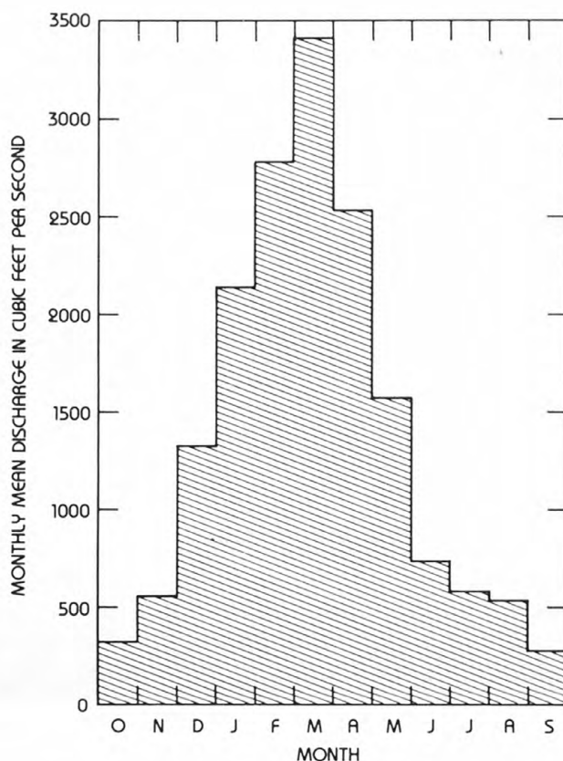
Figure 6.—Monthly mean discharge (1934–77) at gaging station 03214000 Tug Fork near Kermit, West Virginia.
