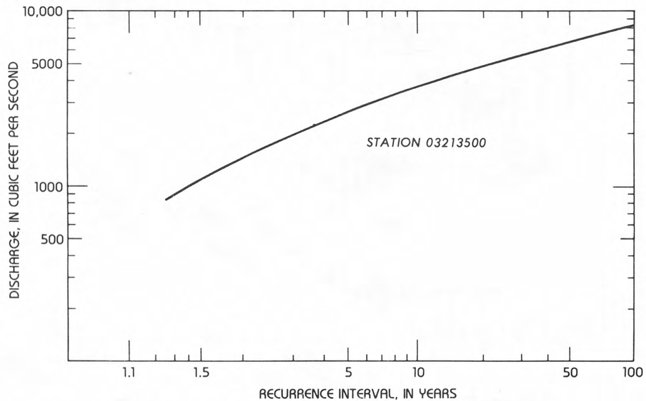
Figure B-2.—Flood-frequency curve for station 03213500 Panther Creek near Panther, West Virginia.
