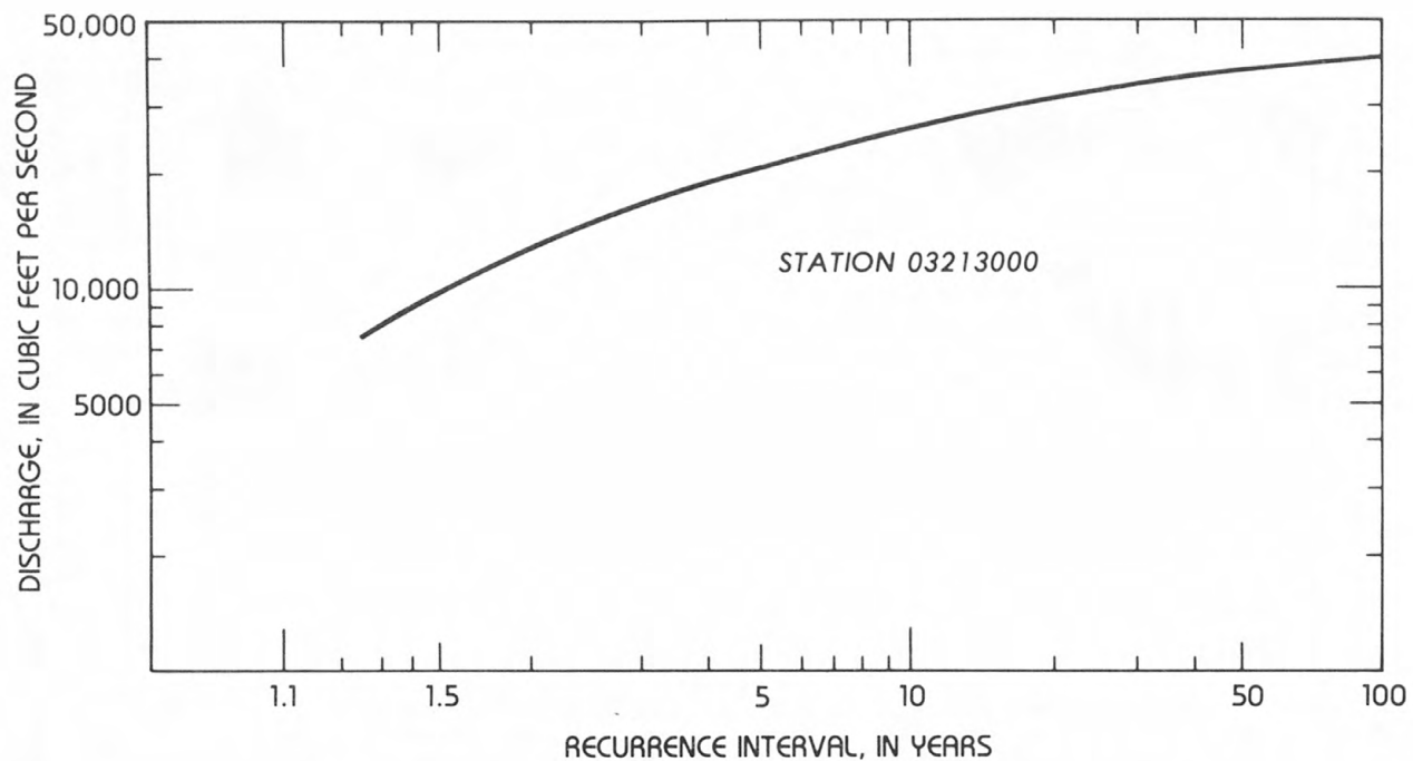
Figure B-1.—Flood-frequency curve for station 03213000 Tug Fork at Litwar, West Virginia.
