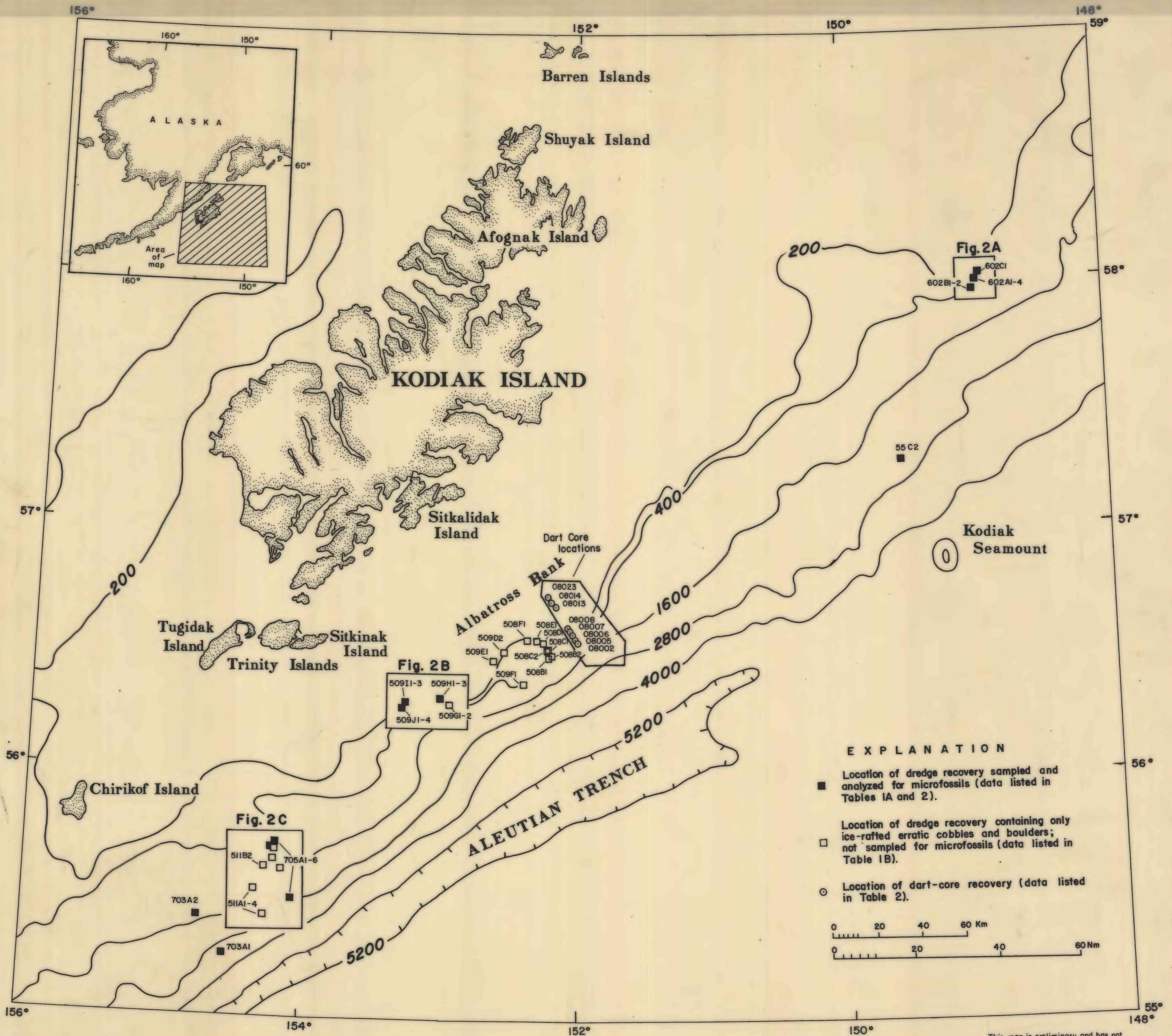
Figure 1. Geography of the Kodiak shelf showing locations of sites that were dredged and dart cored during 1979.
