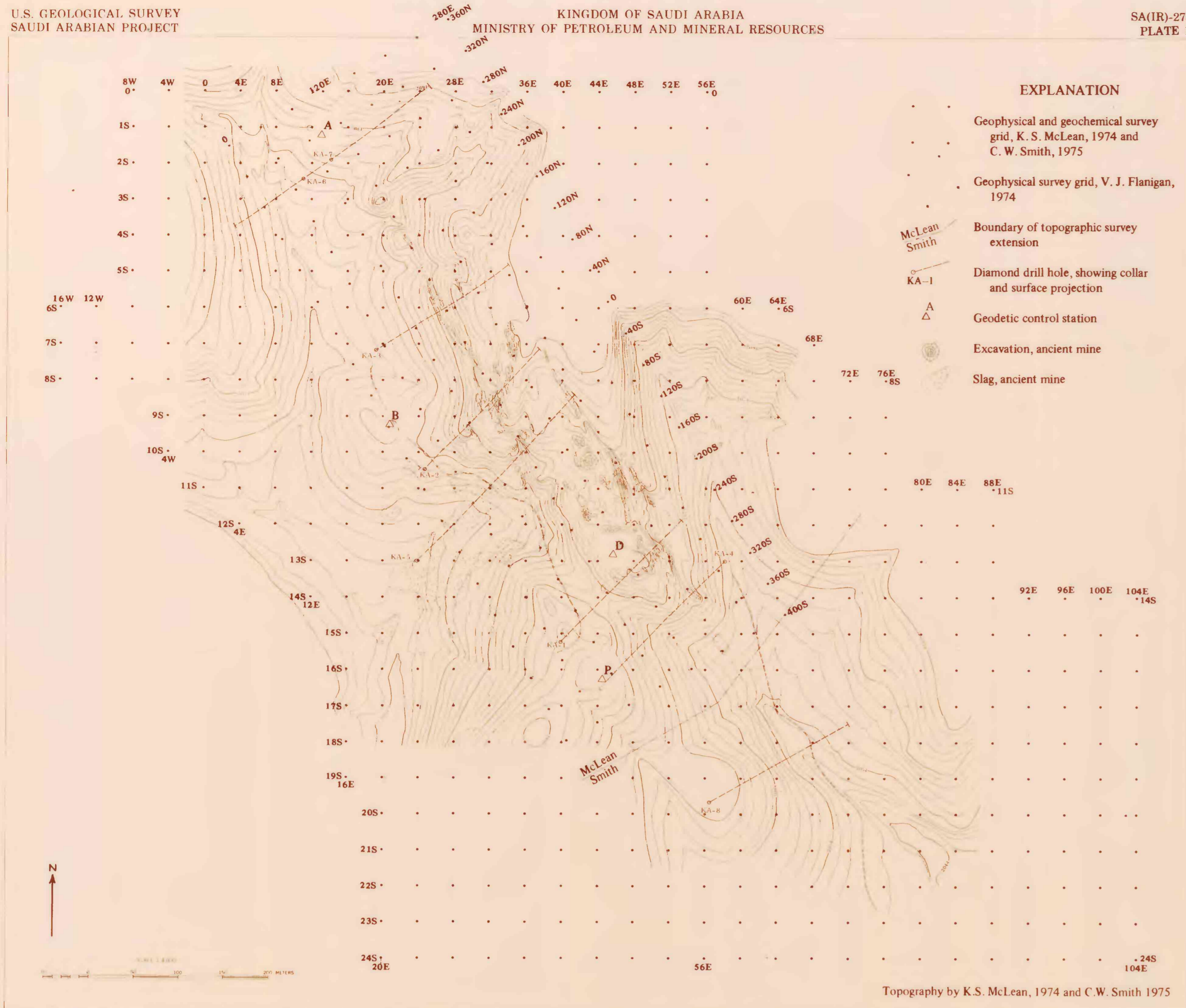
TOPOGRAPHIC MAP OF KUTAM MINE, KINGDOM OF SAUDI ARABIA, SHOWING GRIDS USED IN GEOCHEMICAL AND GEOPHYSICAL SURVEYS
