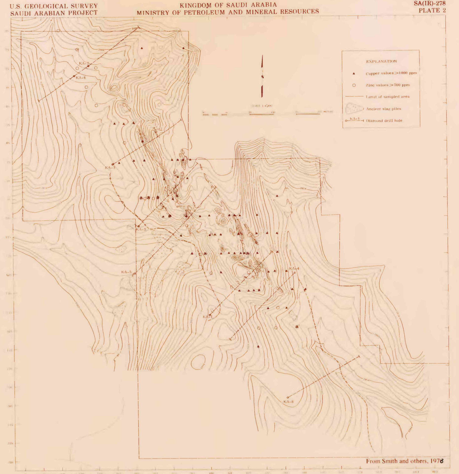
TOPOGRAPHIC AND GEOCHEMICAL MAP OF THE KUTAM MINE, KINGDOM OF SAUDI ARABIA, SHOWING SAMPLE LOCATIONS ANOMALOUS IN COPPER AND ZINC
