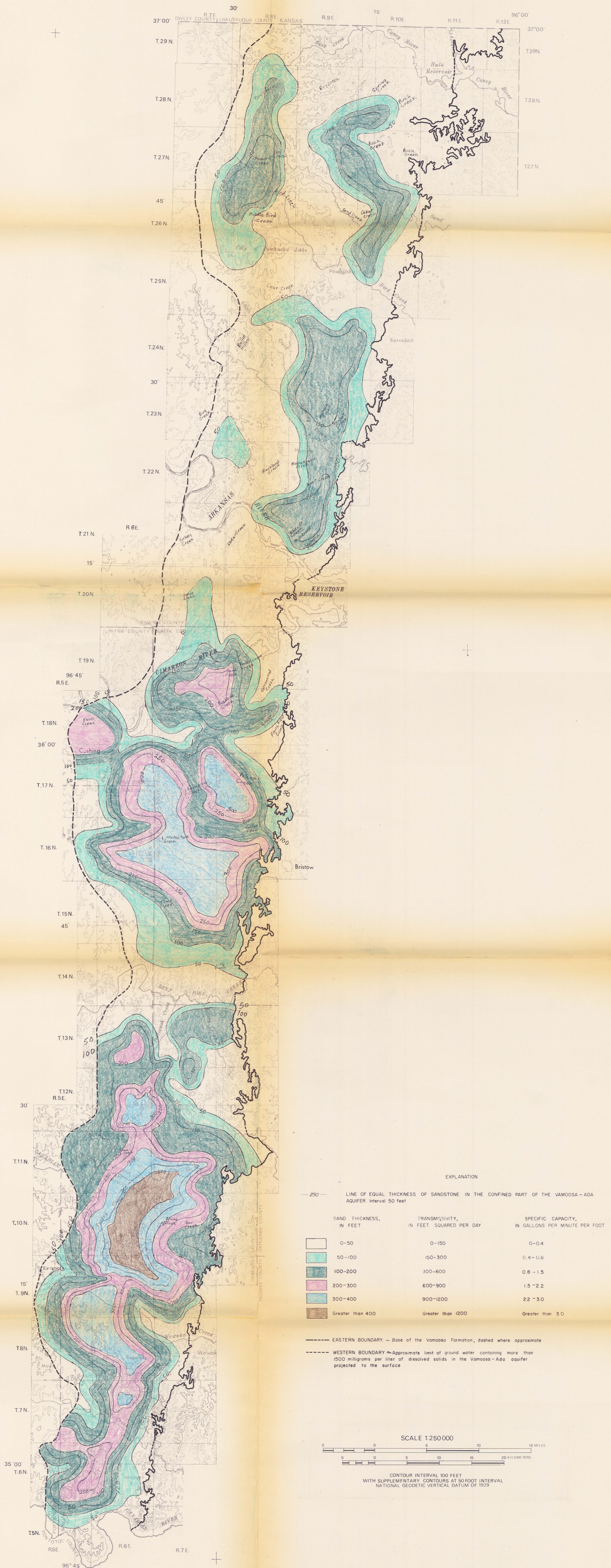
Figure 3-- Map showing aggregate sandstone thickness, theoretical transmissivity, and theoretical specific capacities of wells for the confined part of the Vamoosa-Ada aquifer, eastcentral Oklahoma.
