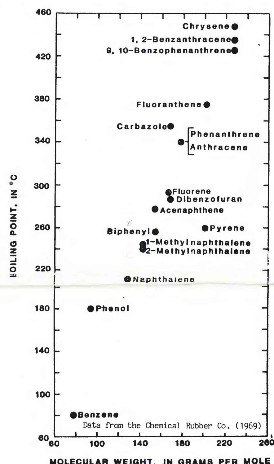
Relationship between boiling point and molecular weight for selected coal-tar compounds
