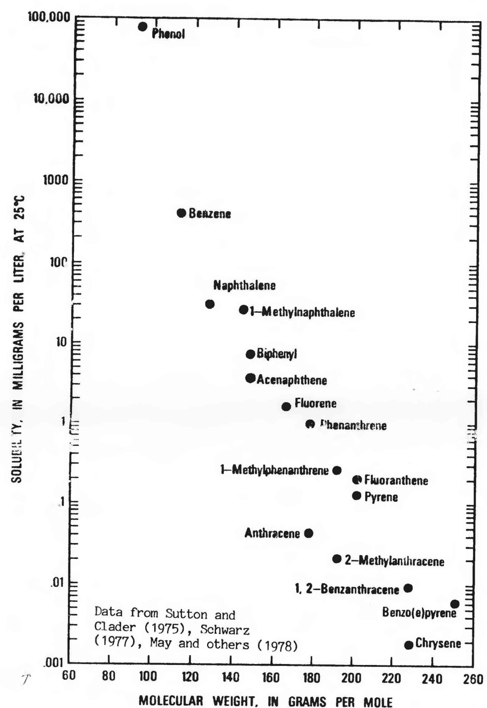
Relationship between solubility and molecular weight for selected coal-tar compounds
