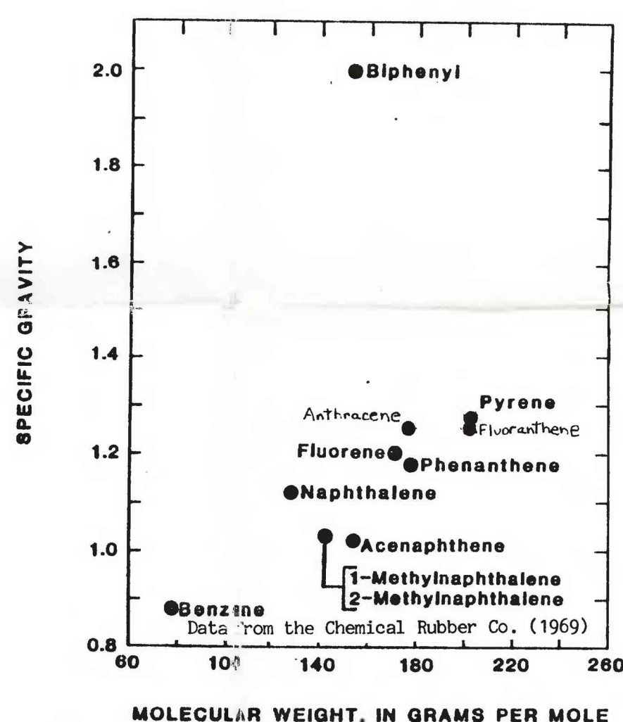
Relationship between specific gravity and molecular weight for selected coal-tar compounds
