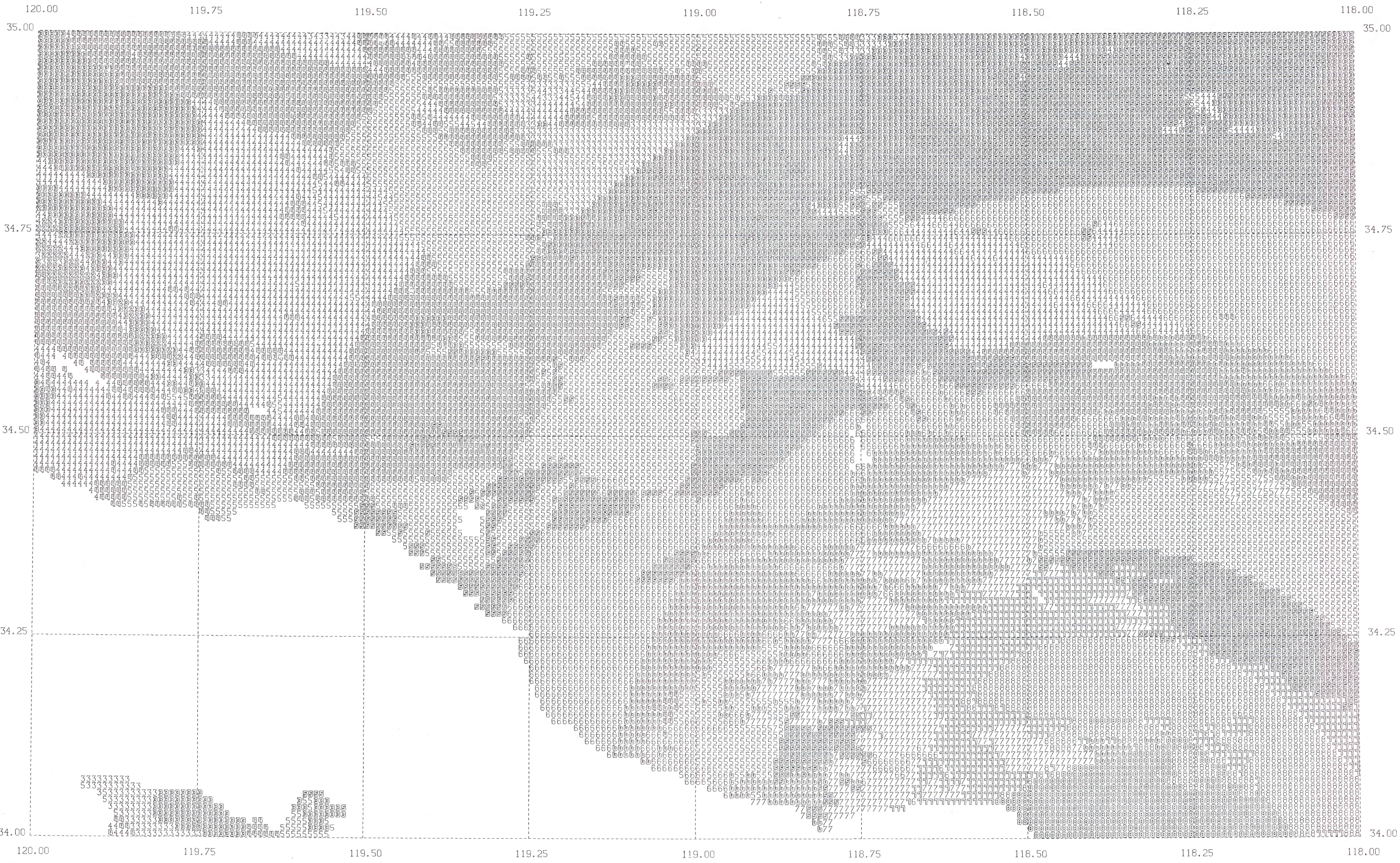
Fig. 7a ROSSI-FOREL INTENSITIES NEWPORT-INGLEWOOD FAULT LOS ANGELES SHEET
