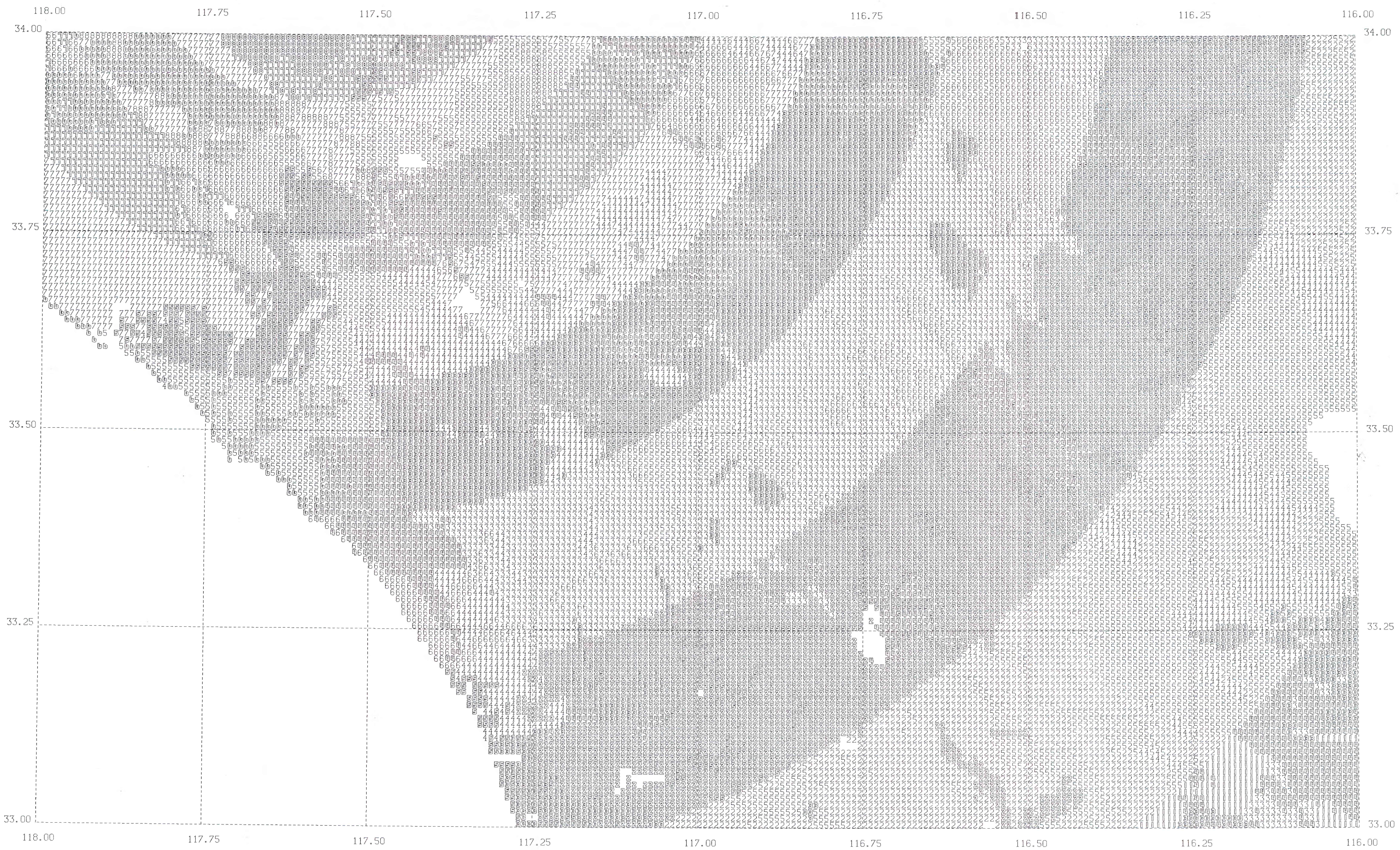
Fig. 9b ROSSI-FOREL INTENSITIES CUCAMONGA FAULT SANTA ANA SHEET
