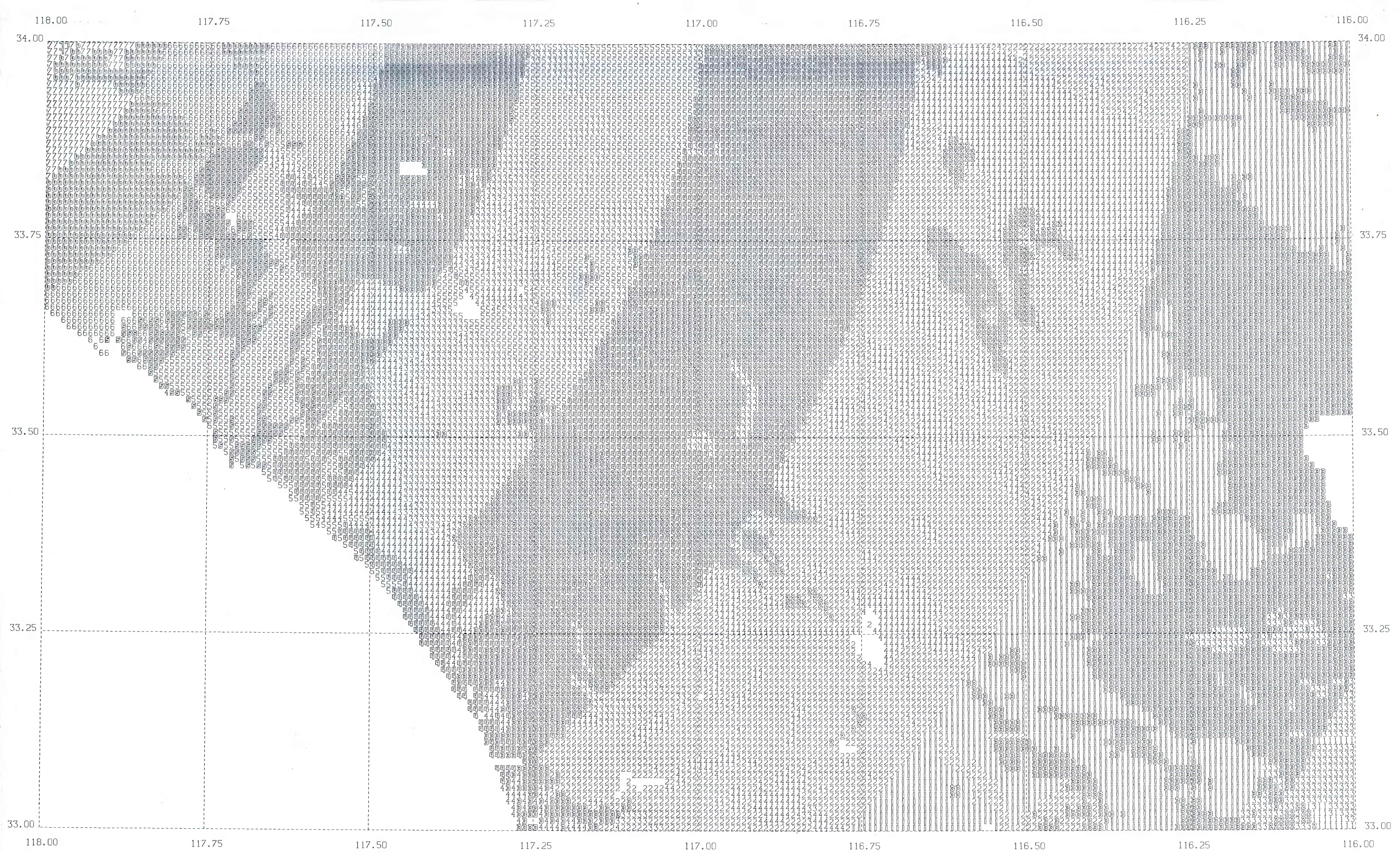
Fig. 10c ROSSI-FOREL INTENSITIES SANTA MONICA FAULT SANTA ANA SHEET
