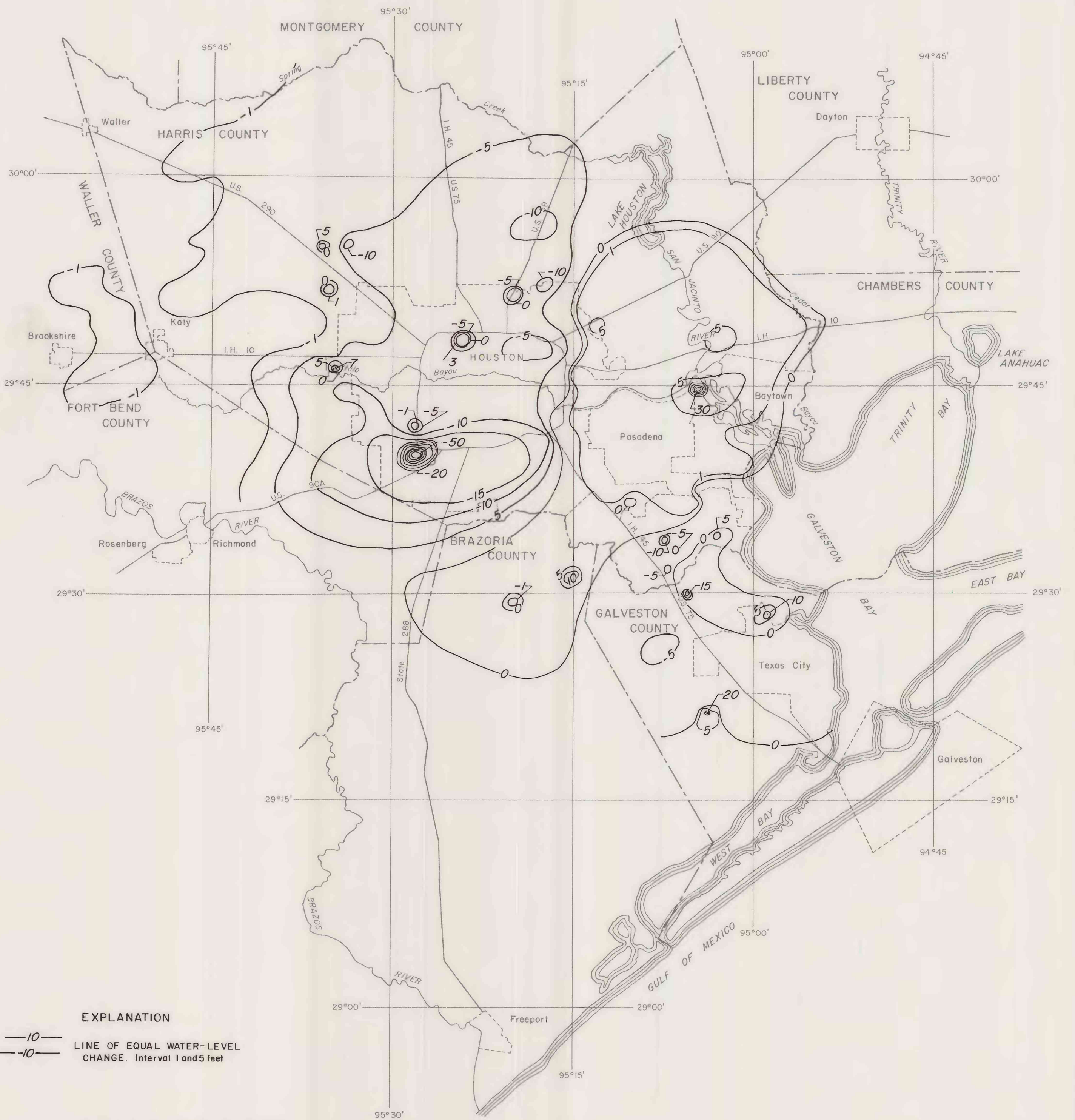
FIGURE 2.—APPROXIMATE WATER-LEVEL CHANGES IN WELLS IN THE CHICOT AQUIFER IN THE HOUSTON-GALVESTON REGION, TEXAS, 1980-81
