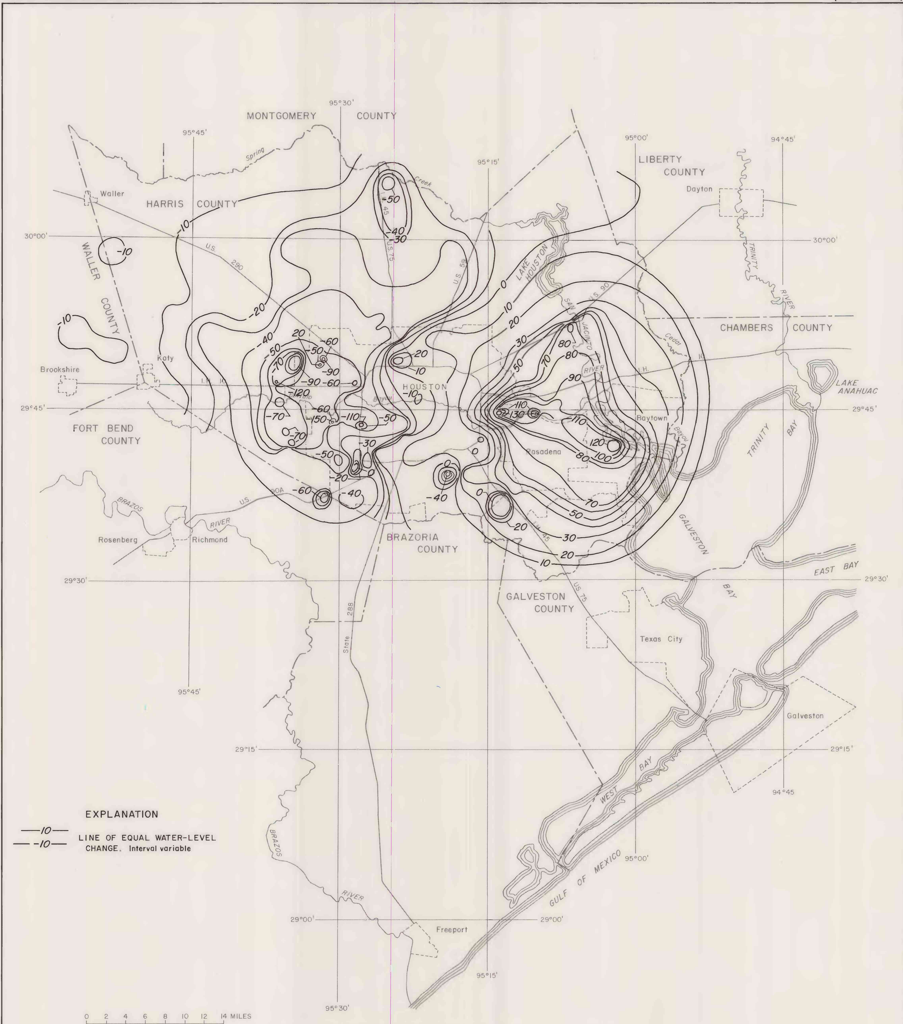
FIGURE 3.—APPROXIMATE WATER-LEVEL CHANGES IN WELLS IN THE EVANGELINE AQUIFER IN THE HOUSTON-GALVESTON REGION, TEXAS, 1977-81
