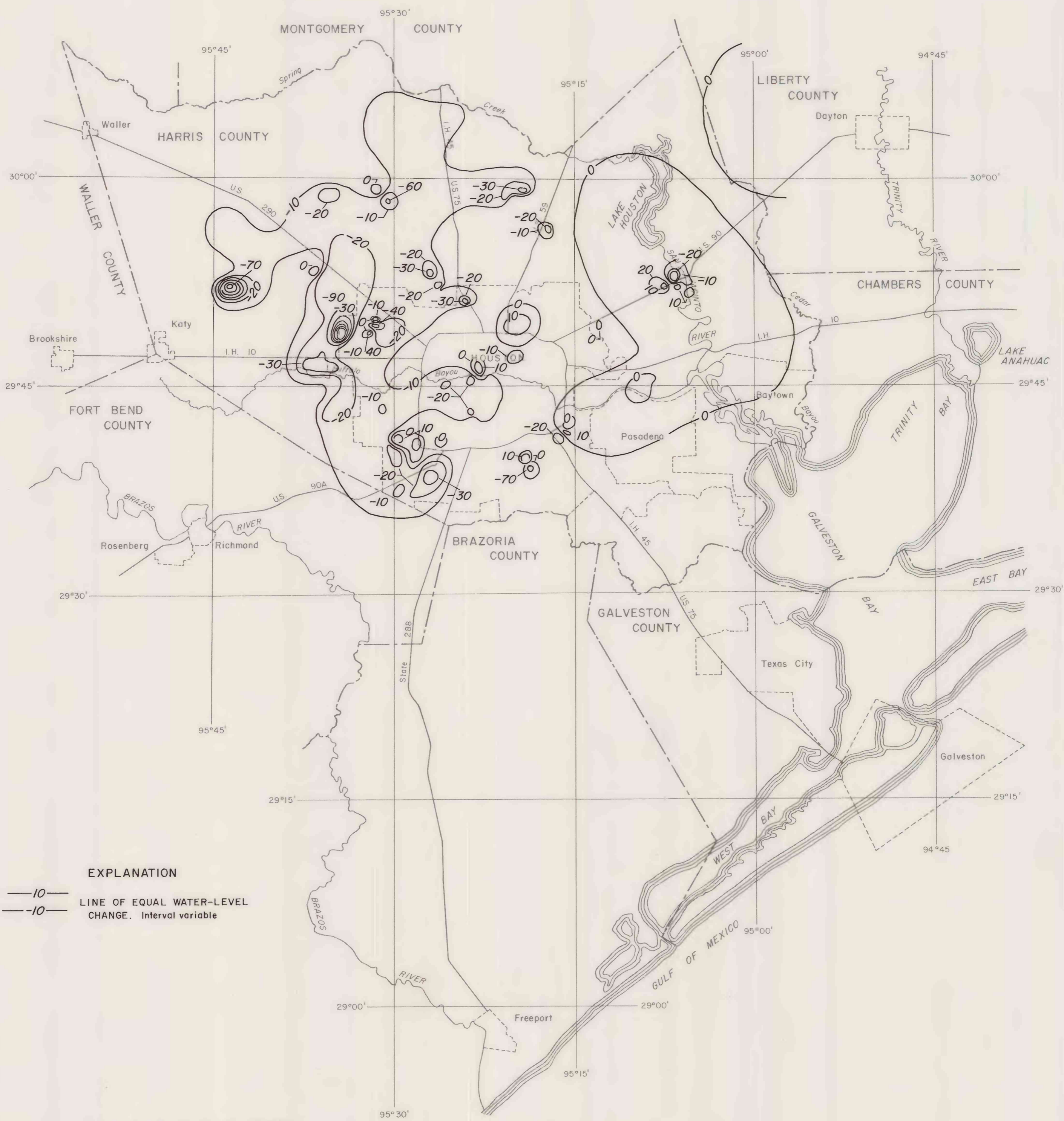
FIGURE 4.—APPROXIMATE WATER-LEVEL CHANGES IN WELLS IN THE EVANGELINE AQUIFER IN THE HOUSTON-GALVESTON REGION, TEXAS, 1980-81
