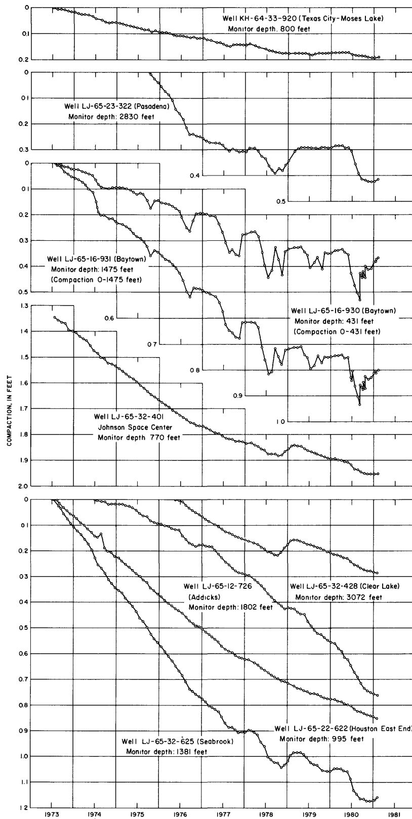
FIGURE 5.-MEASURED COMPACTION, 1973-81, IN THE HOUSTON-GALVESTON REGION, TEXAS
