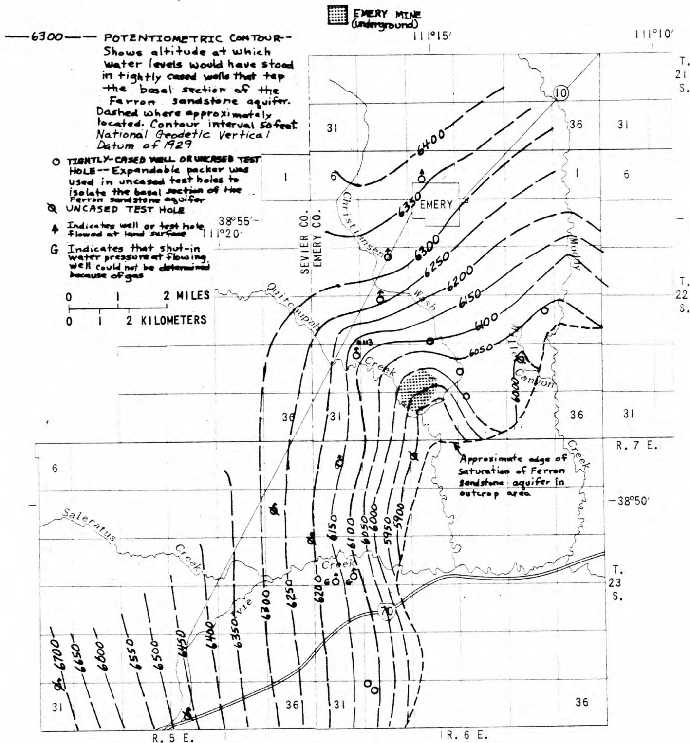
Figure 11.-- Potentiometric surface of the basal section of the Ferron sandstone aquifer in the Emery area, 1979.
