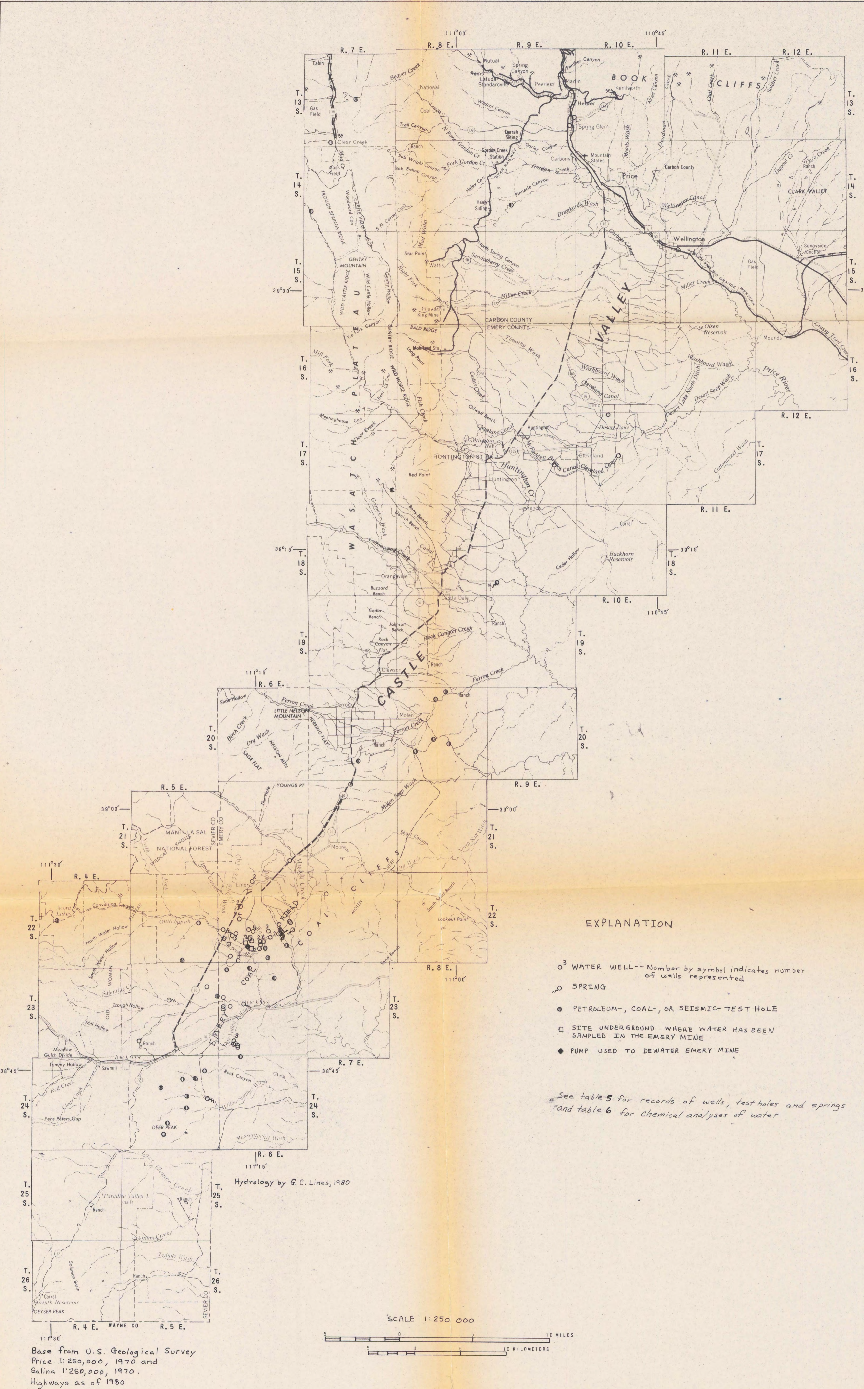
Figure 2.--Map showing location of selected wells, springs, and test holes in and near Castle Valley, Utah, where ground-water information is available, 1980.
