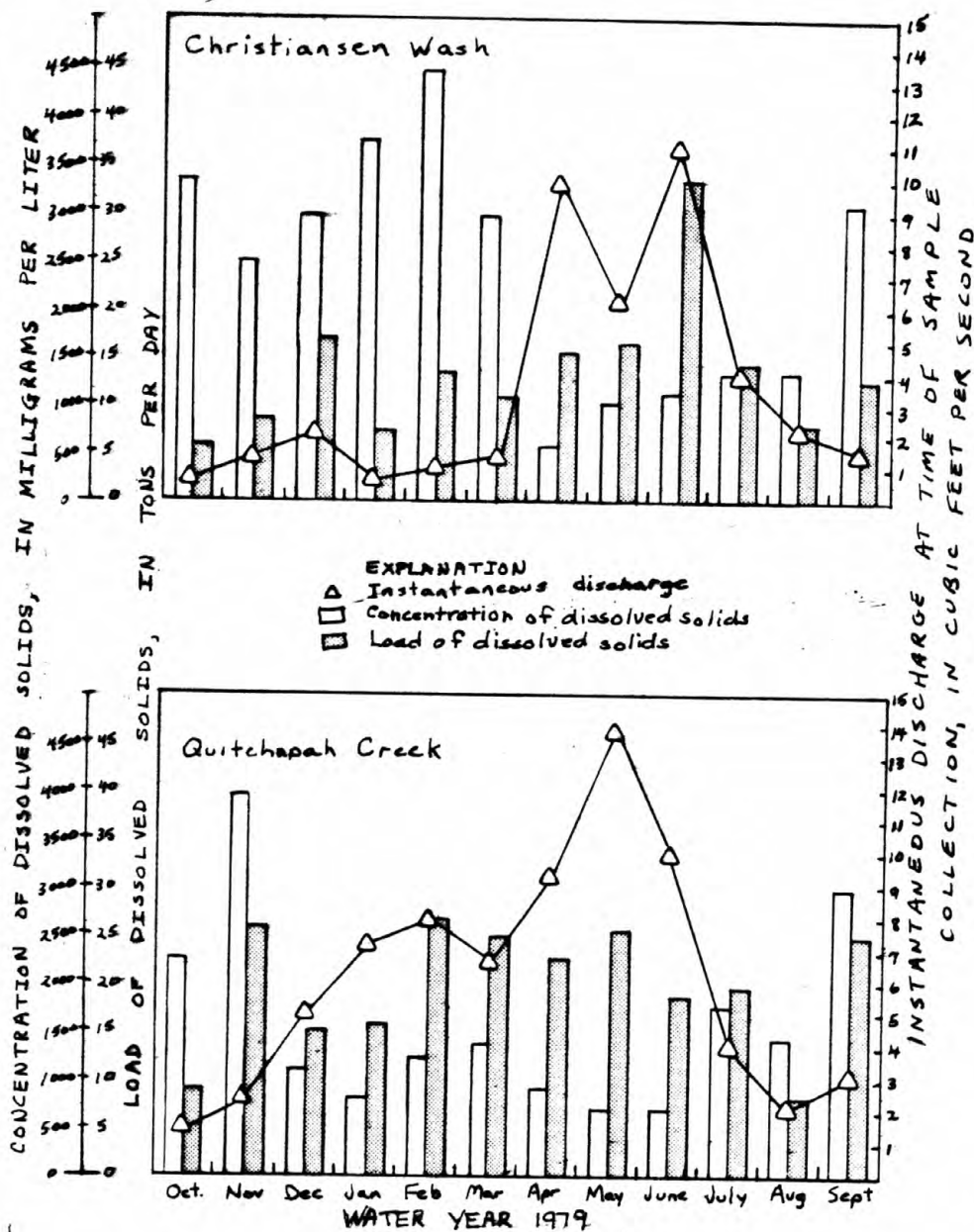
Figure 20.-- Monthly variation in the concentration and load of dissolved solids at gaging stations 09331900 and 09331950 on Quitchapah Creek and Christiansen Wash in the Emery area, water year 1979.
