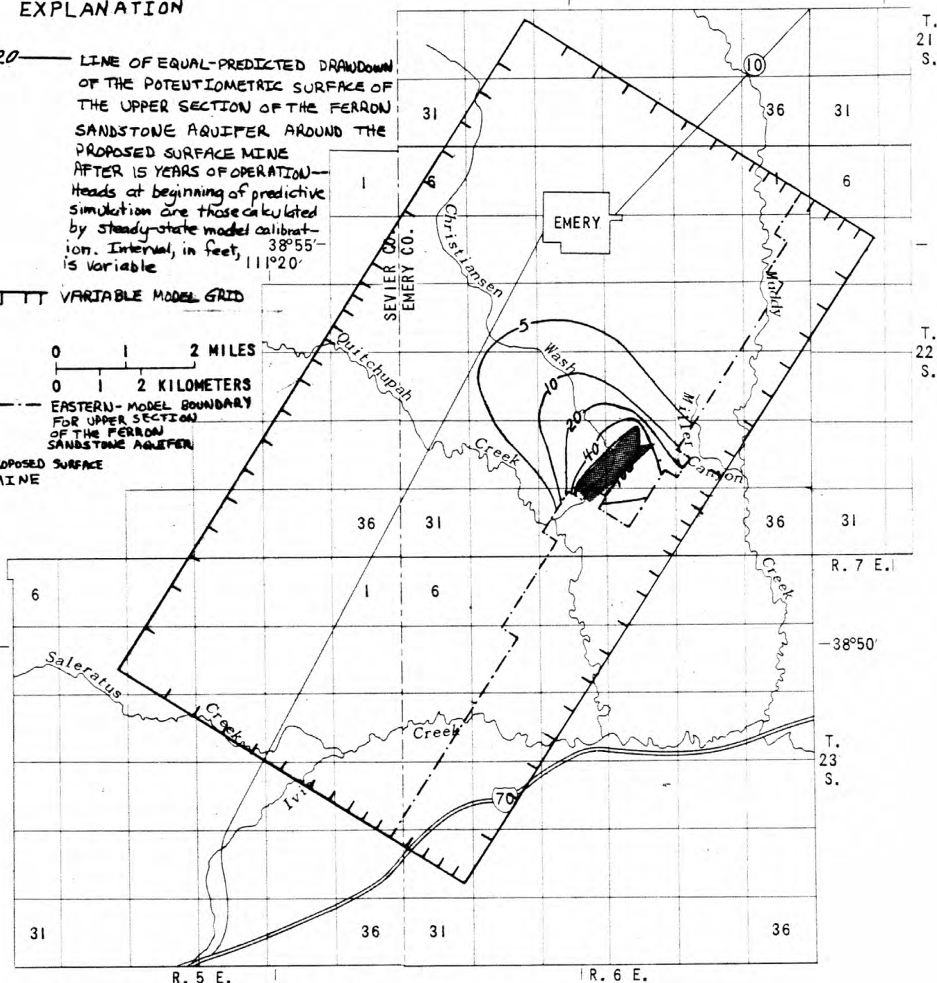
Figure 23. -- Variable grid used in the three-dimensional digital-computer model and the predicted drawdown of the potentiometric surface of the upper section of the Ferron sandstone aquifer around the proposed surface mine after 15 years of operation.
