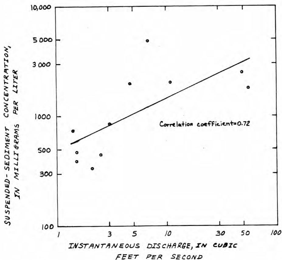
Figure 22.-- Relationship between suspended-sediment concentration and stream discharge at gaging station 09331950 on Christiansen Wash in the Emery area, May 1978 - September 1979.
