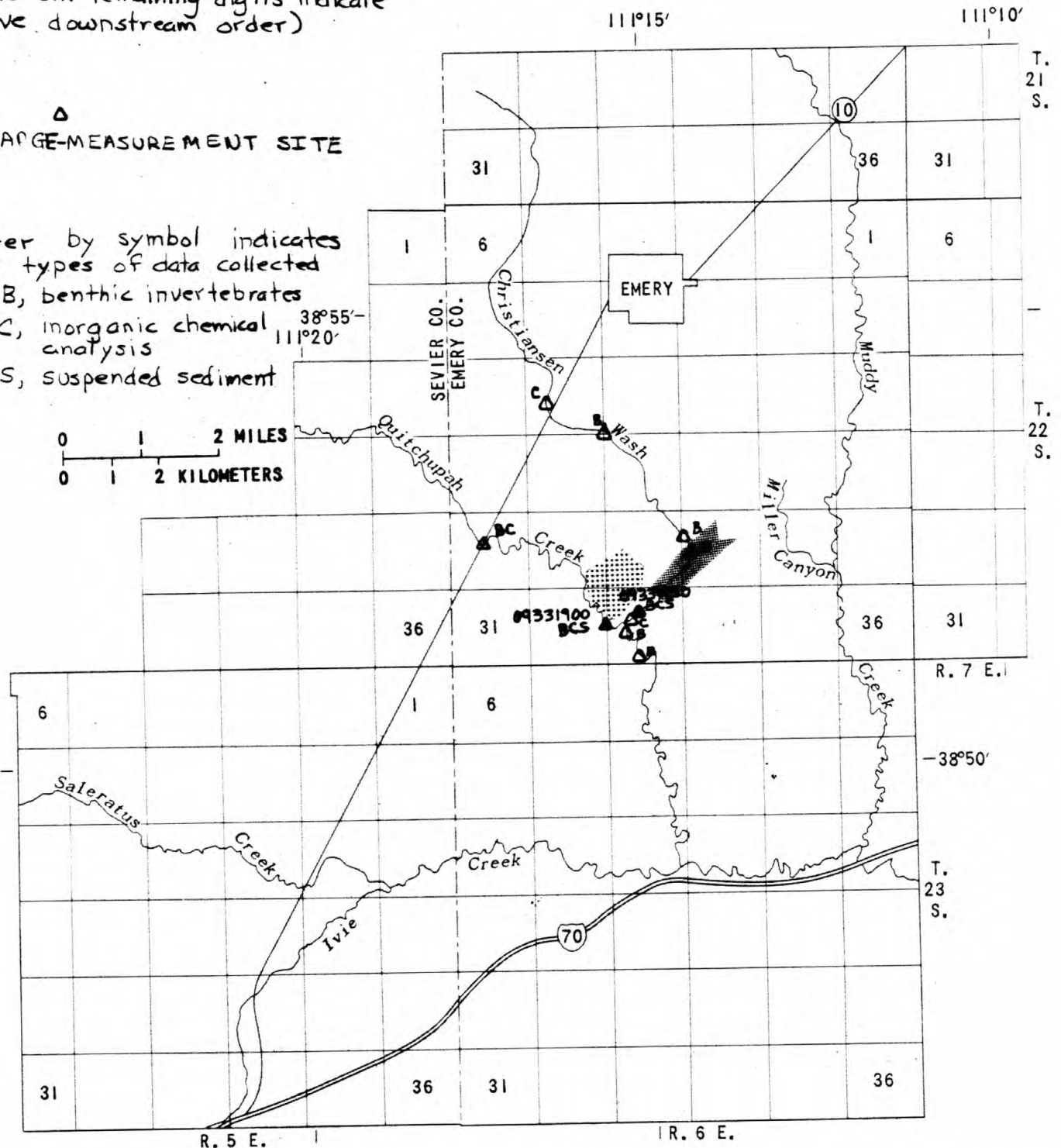
Figure 19.-- Location of data-collection sites on Quitchupeh Creek and Christiansen Wash in the Emery area 1978-79.
