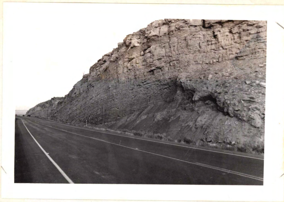
Figure 7.--Outcrop of the Washboard Unit of Cotter (1975a) of the Ferron Sandstone Member of the Mancos Shale along U.S. Highway 6 southeast of Wellington.
