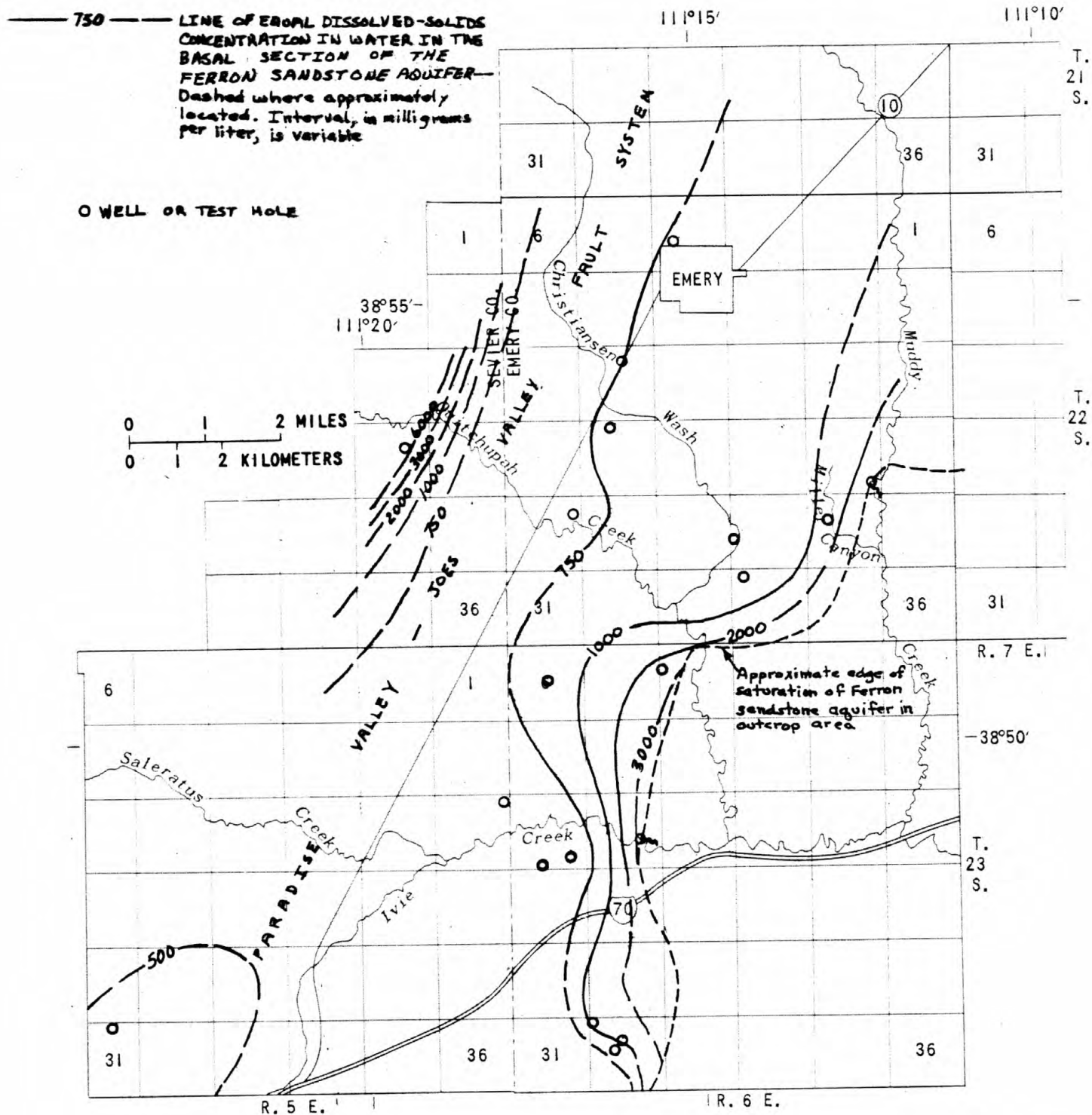
Figure 17.-- Concentration of dissolved solids in water in the basal section of the Ferron sandstone aquifer in the Emery area, 1979.
