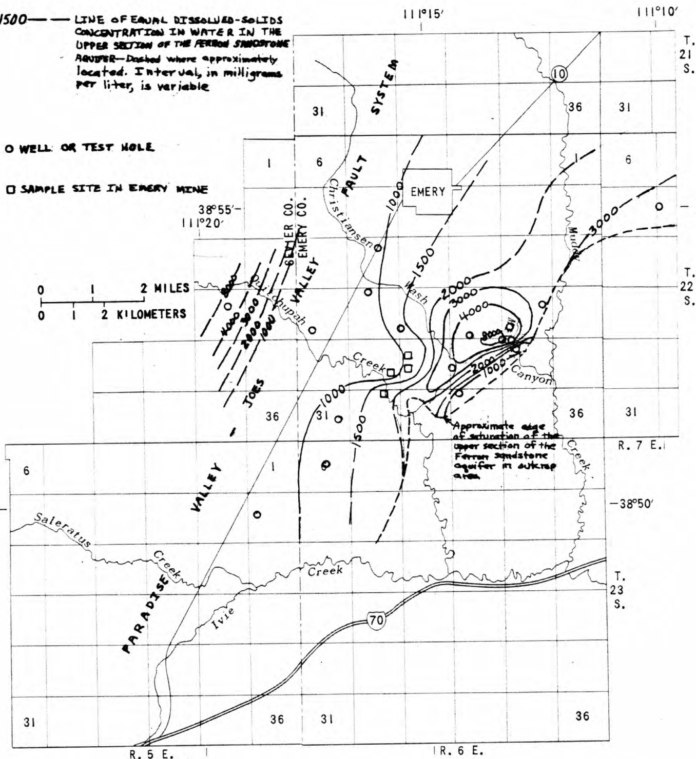
Figure 18.— Concentration of dissolved solids in water in the upper section of the Ferron sandstone aquifer in the Emery area, 1979.
