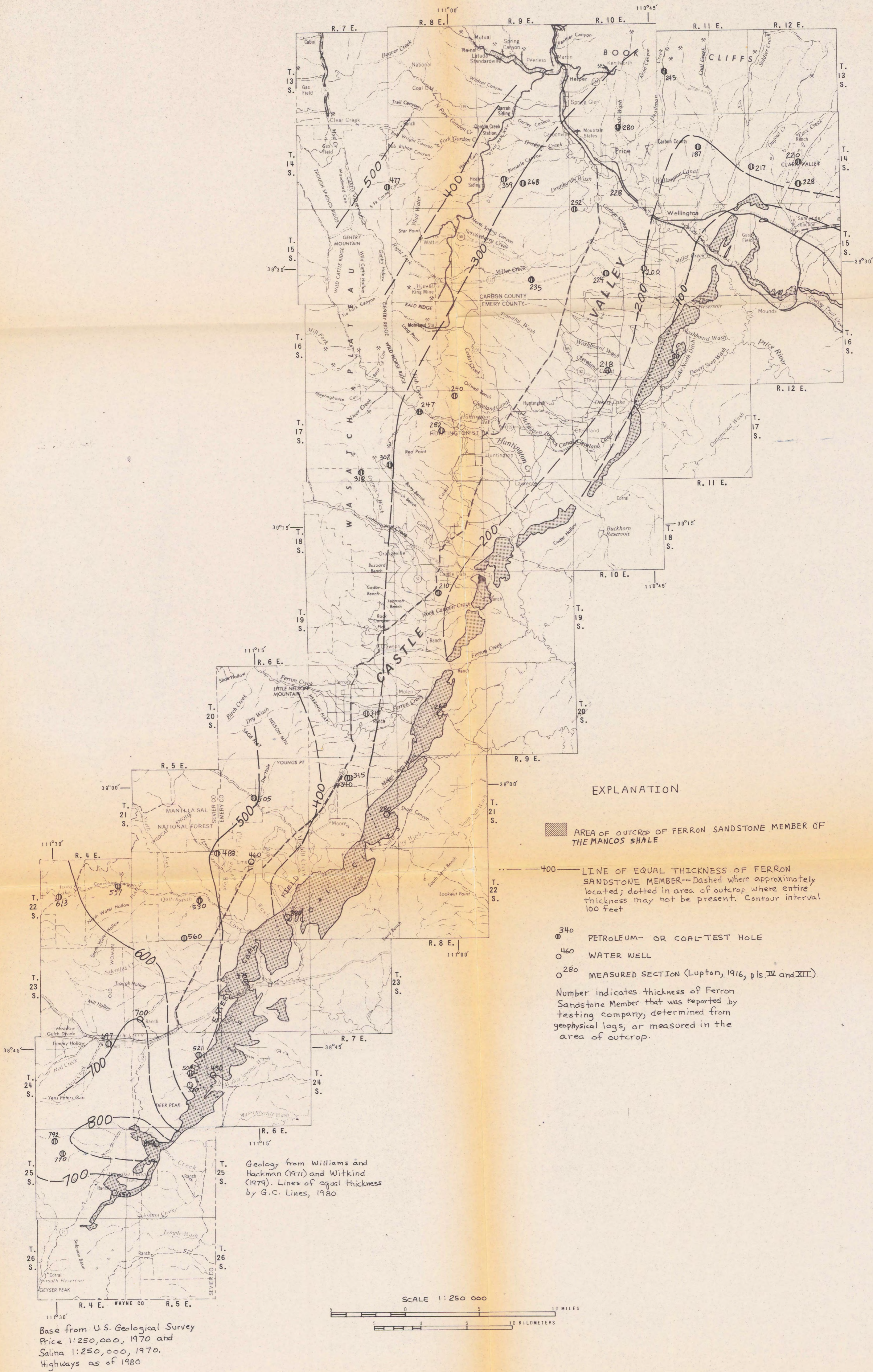
Figure 4. --Map showing thickness of the Ferron Sandstone Member of the Mancos Shale in Castle Valley, Utah.
