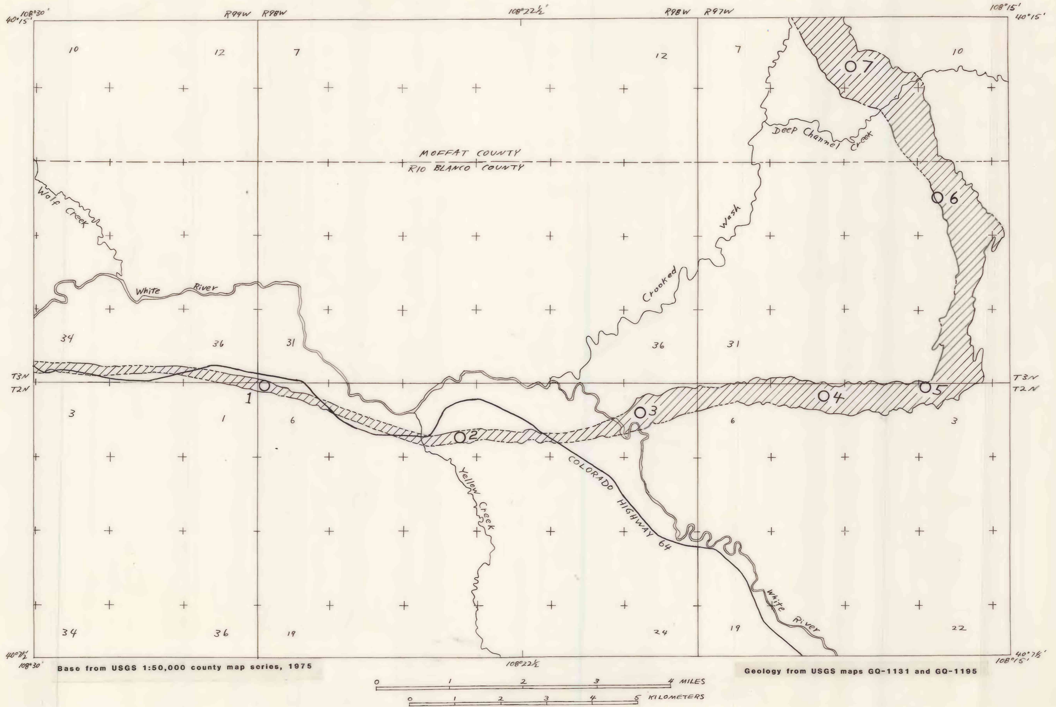
PLATE 1. -- Outcrop of the upper member of the Fort Union Formation (diagonal lines), southern part of the Crooked Wash area. Numbered circles are uranium occurrences
