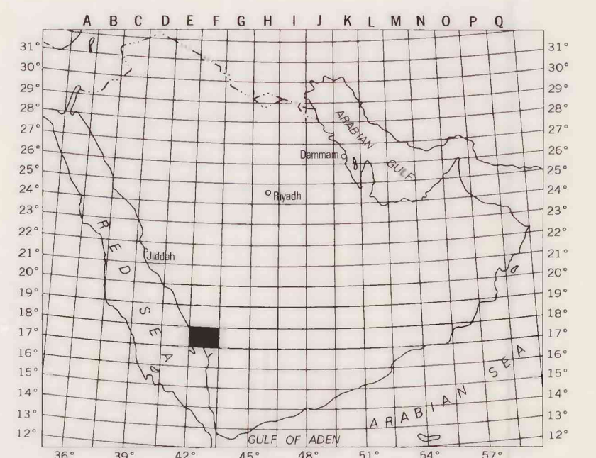
Index to 1:250,000-scale Landsat image maps of the Arabian Peninsula showing location of the Wādi Baysh Quadrangle, 17F
