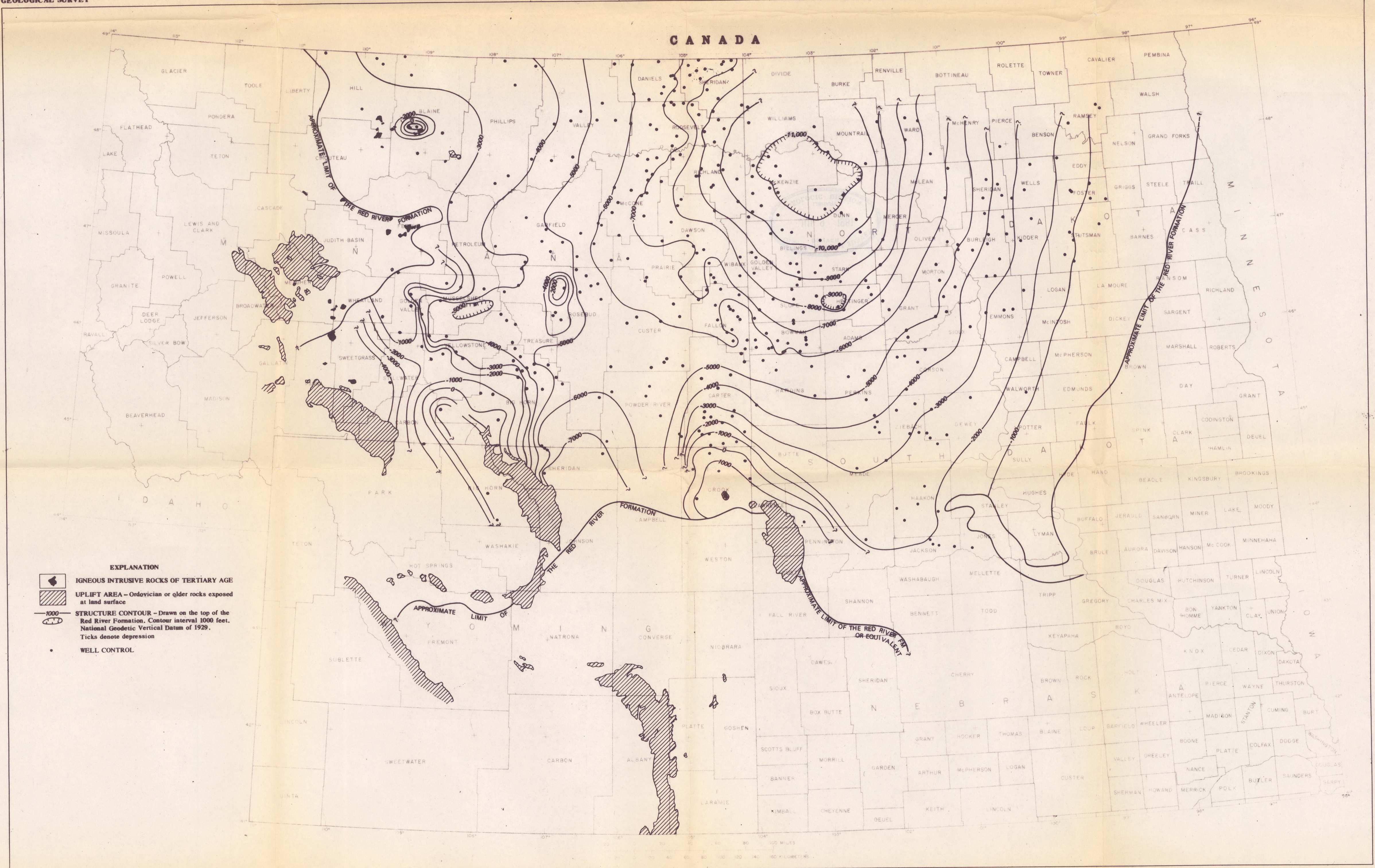
MAP SHOWING ALTITUDE AND CONFIGURATION OF THE TOP OF THE RED RIVER FORMATION (ORDOVICIAN), IN PARTS OF MONTANA, NORTH DAKOTA, SOUTH DAKOTA, AND WYOMING.
