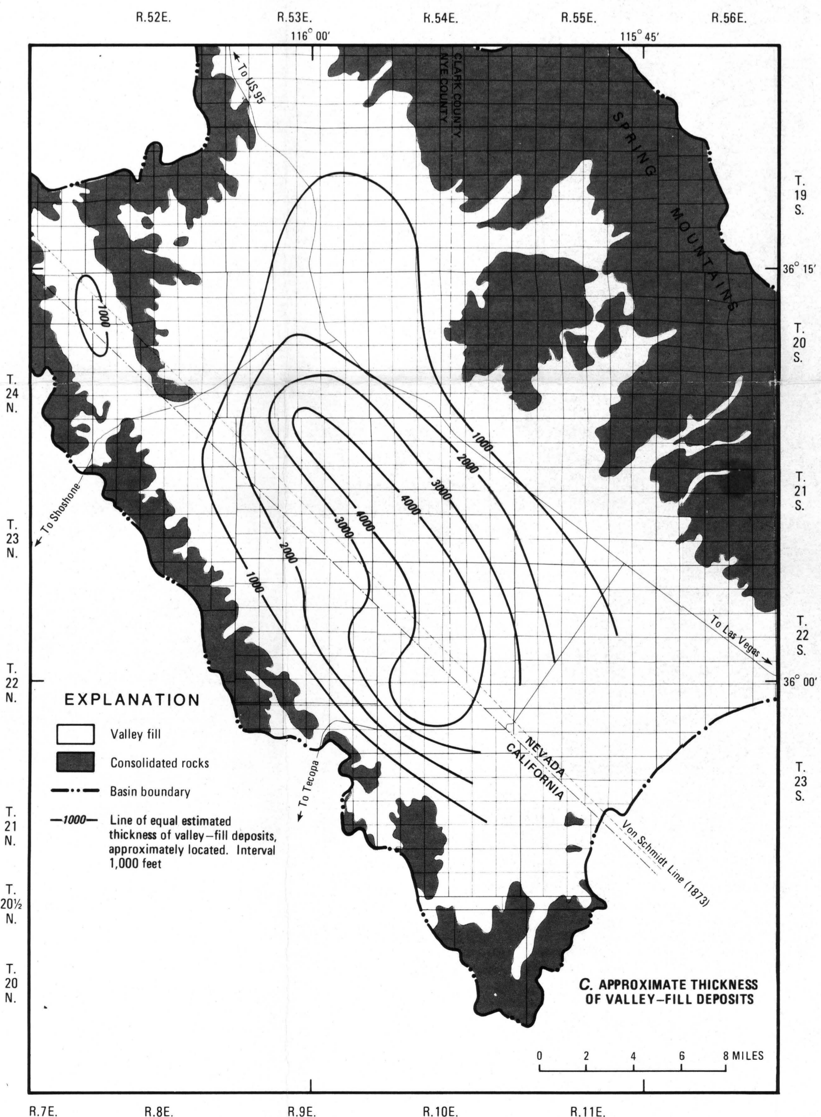
GRAVITY INFORMATION AND THICKNESS OF VALLEY FILL, PAHRUMP VALLEY, NEVADA-CALIFORNIA
