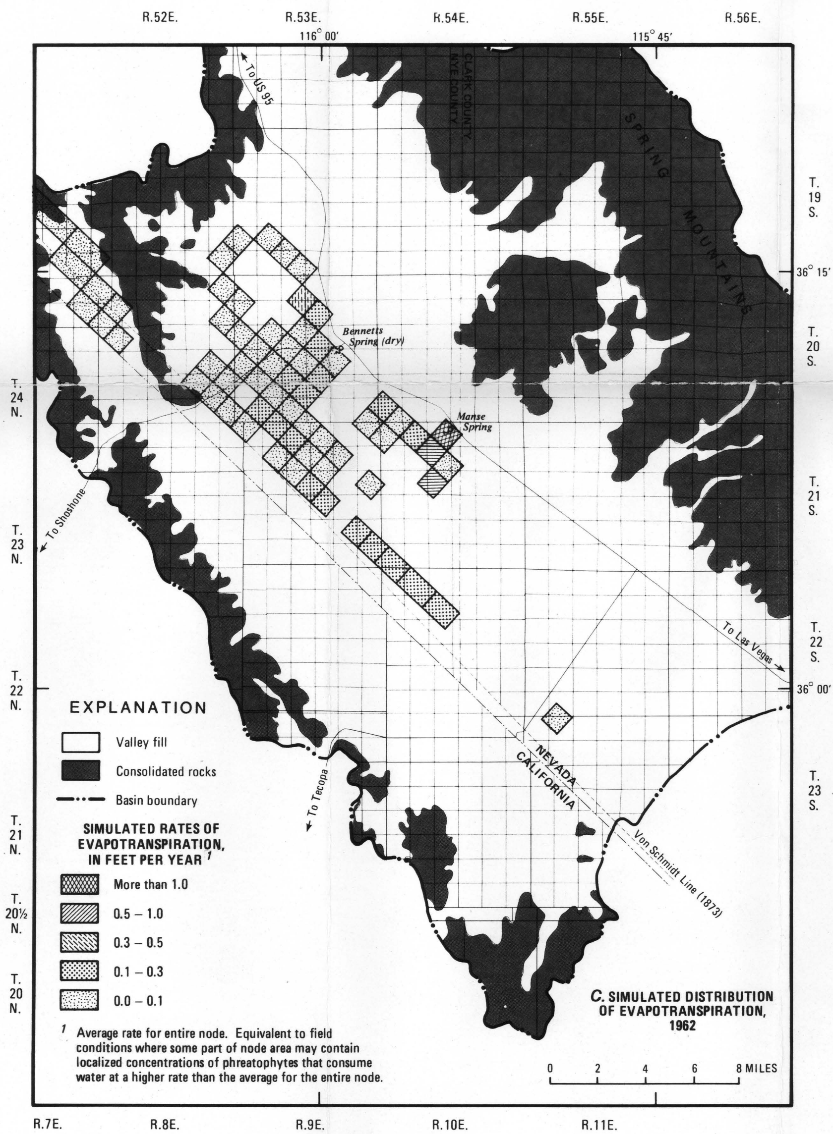
DISTRIBUTION OF PHREATOPHYTES AND SIMULATED DISTRIBUTION OF EVAPOTRANSPIRATION, PAHRUMP VALLEY, NEVADA-CALIFORNIA
