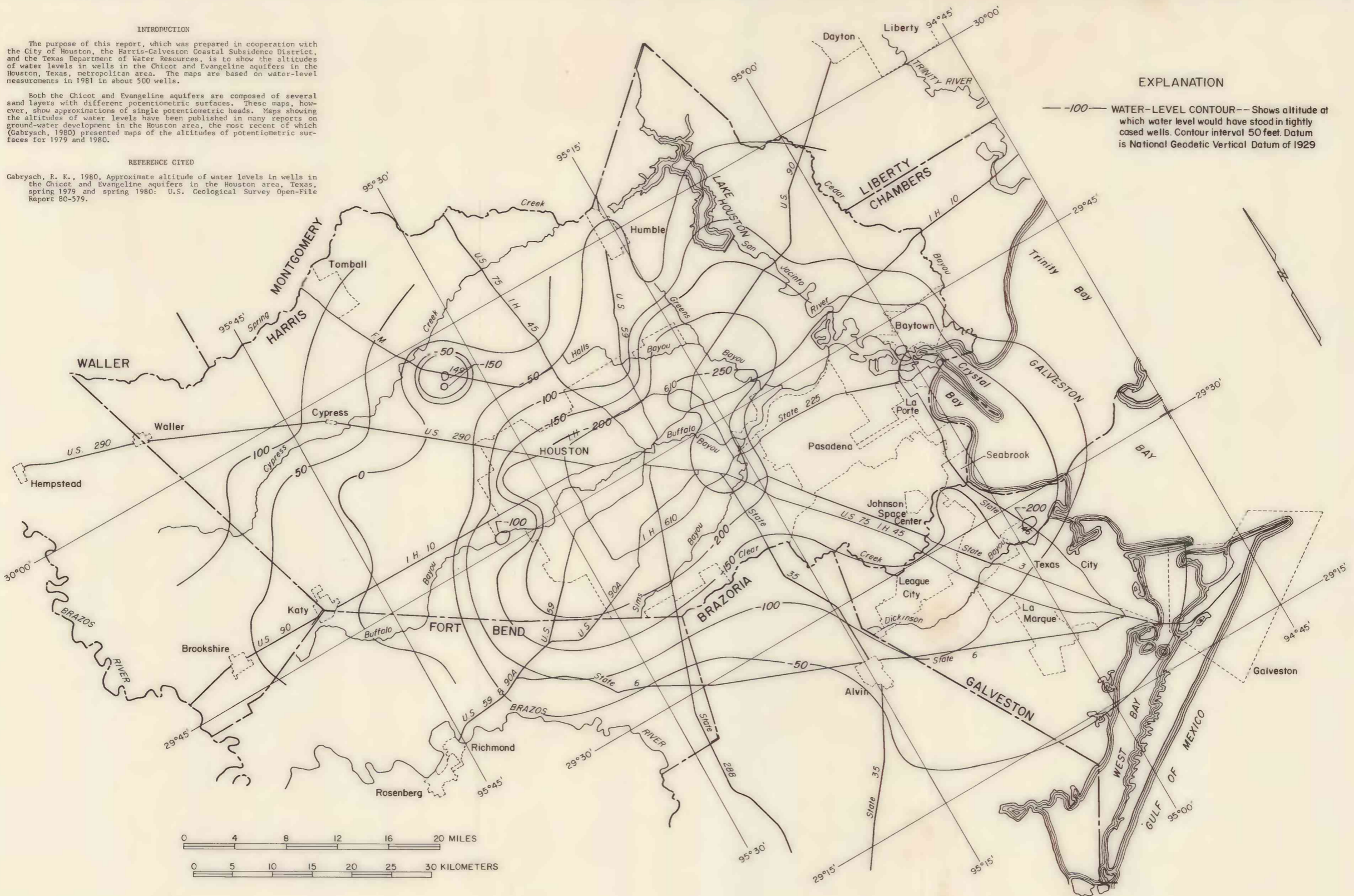
Figure 1.- Approximate altitude of water levels in wells in the Chicot aquifer, Spring 1981
