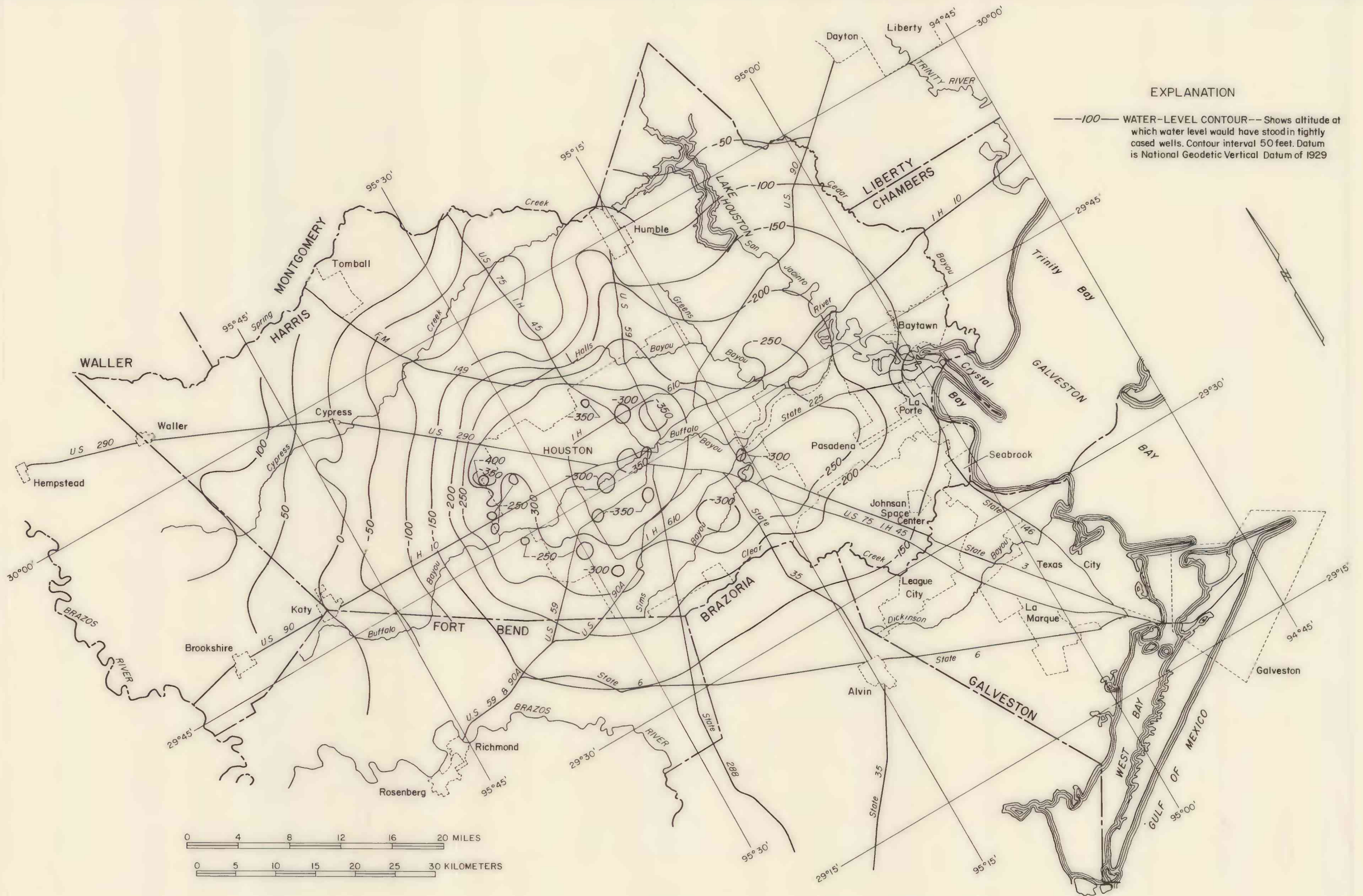
Figure 2.—Approximate altitude of water levels in wells in the Evangeline aquifer, Spring 1981
