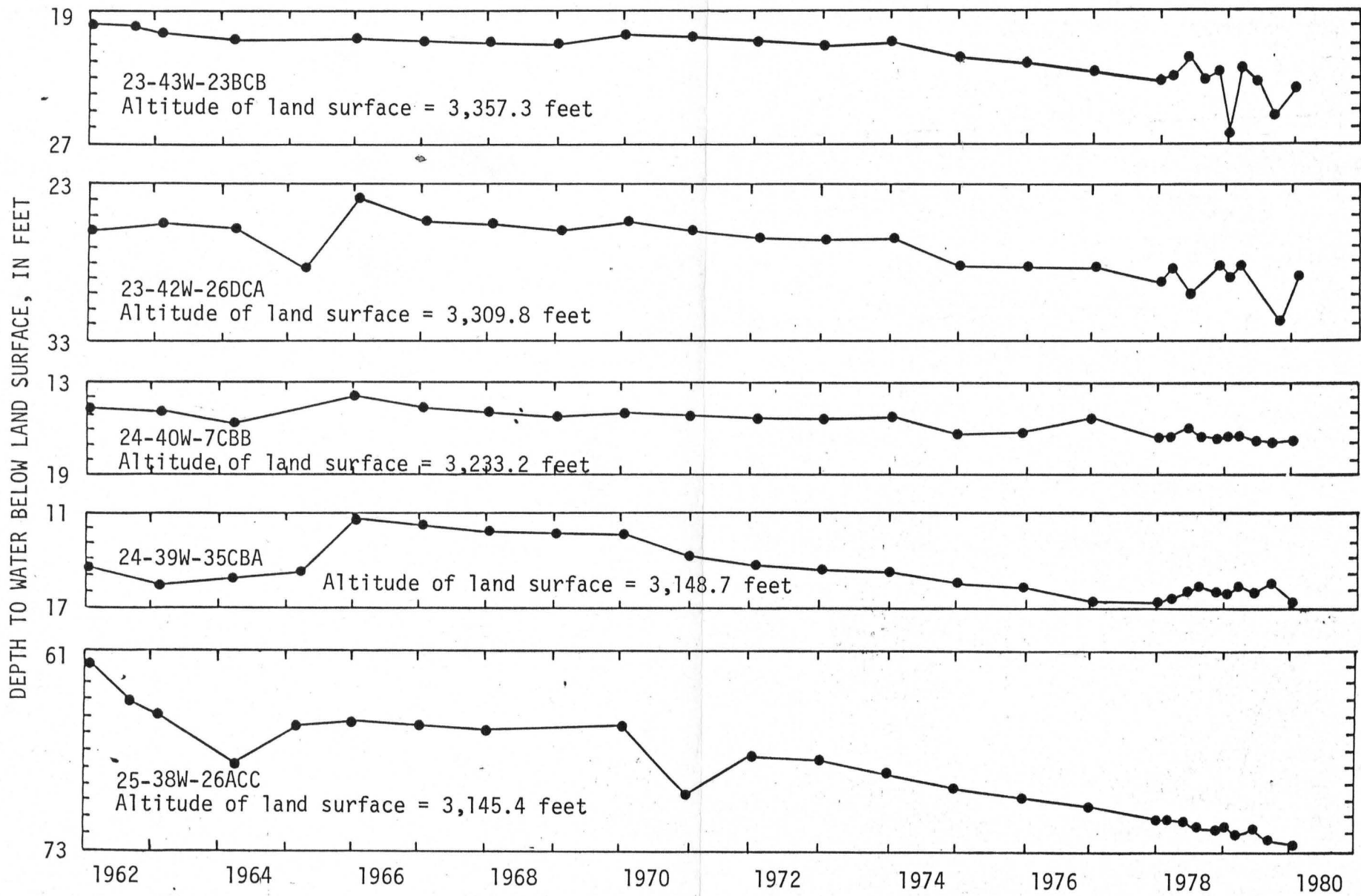
Figure 15.--Water-level fluctuation at selected sites, 1962-79.
