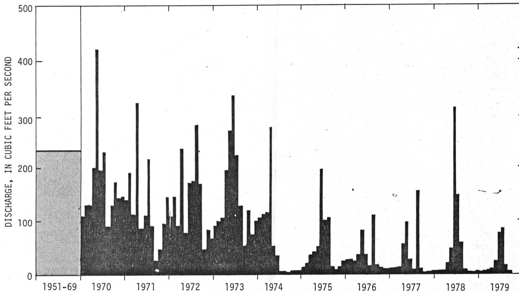
Figure 16.--Monthly discharge of Arkansas River near Coolidge, 1951-69 and 1970-79.
