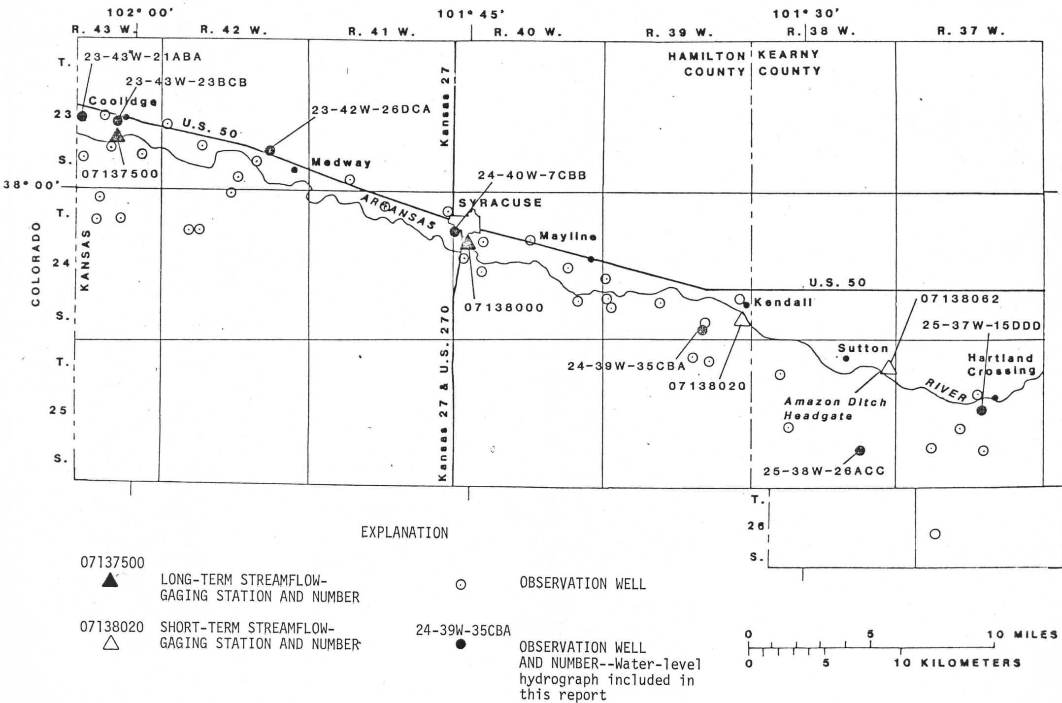
Figure 2.--Location of streamflow-gaging stations and observation wells.
