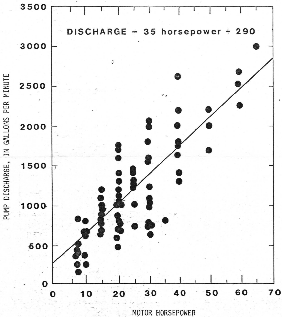
Figure 25.--Relationship between electric-motor horsepower and pump discharge.
