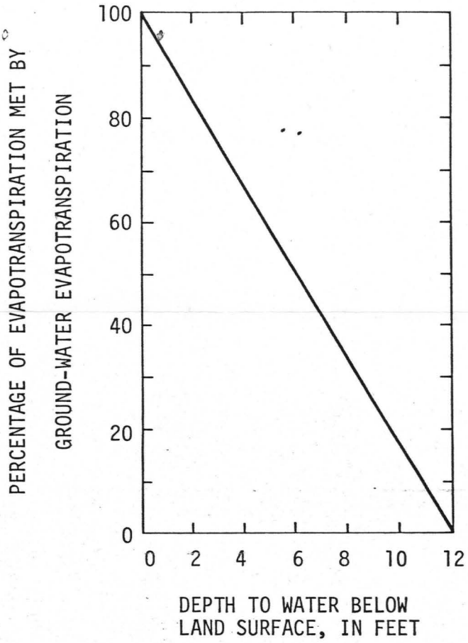
Figure 29.--Relationship between depth to water table and ground-water evapotranspiration.
