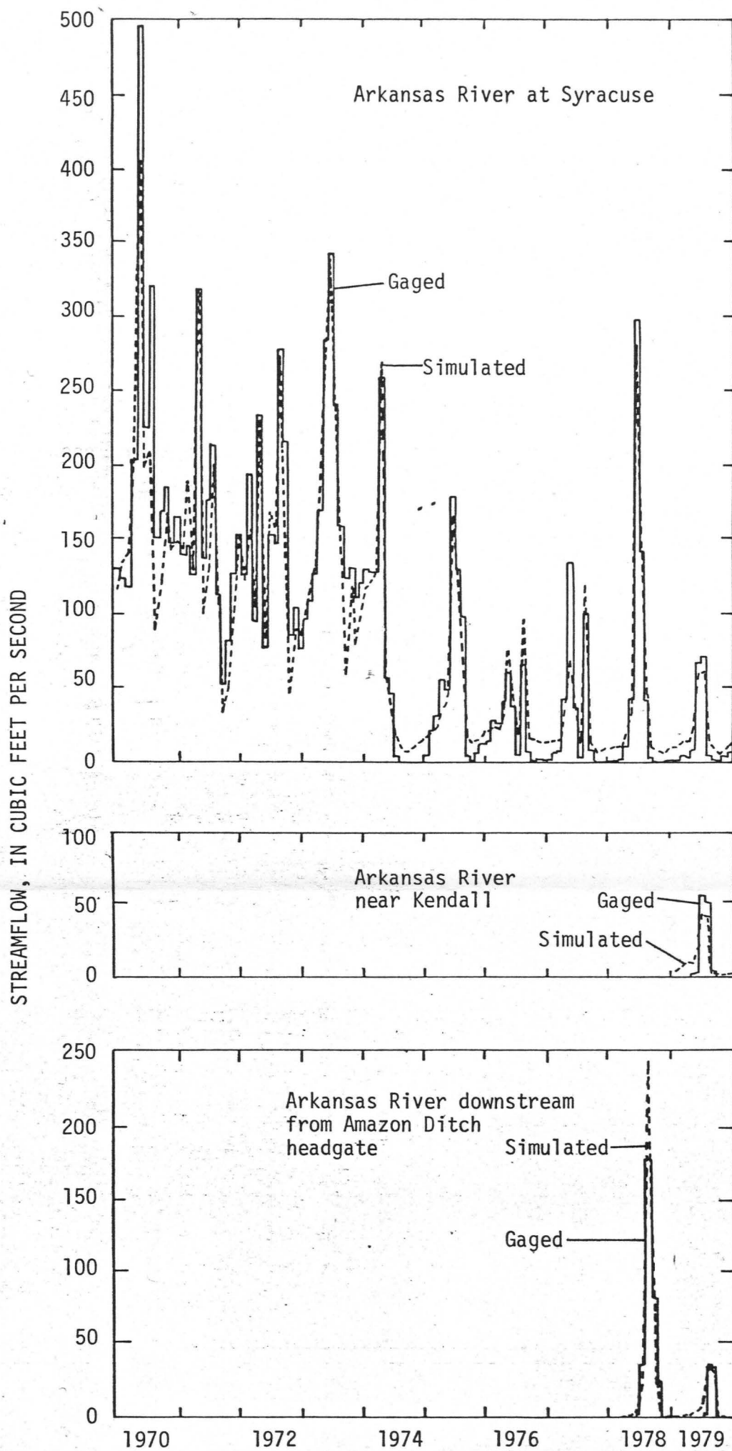
Figure 33.--Gaged and simulated mean monthly discharge of Arkansas River at Syracuse (1970-79), near Kendall (1979), and downstream from Amazon Ditch headgate (1978-79).
